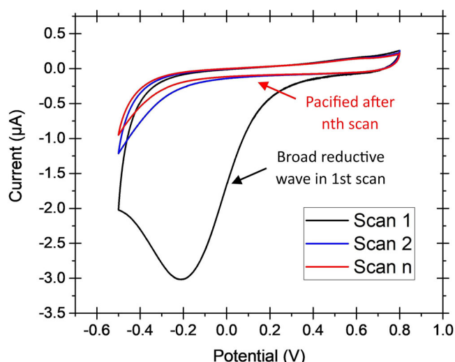
Figure 10. Characteristic cyclic voltammograms for the reduction of an aryl diazonium salt generated in situ from 2-(4-aminobenzyl)isoindoline-1,3-dione. Potential vs. Ag/AgCl (3 M KCl), scan rate 20 mV s -1 , GC working electrode. Solvent system 1:5 water/acetonitrile + 0.1 M Bu 4 NPF 6 + 0.5% v/v 6.6 M HCl. Ambient temperature.
