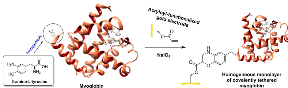
Figure 15. Covalent crosslinking of myoglobin to a gold electrode as a homogeneous monolayer, through the incorporation and Diels–Alder reaction of a 3-amino-L-tyrosine residue. [218]
