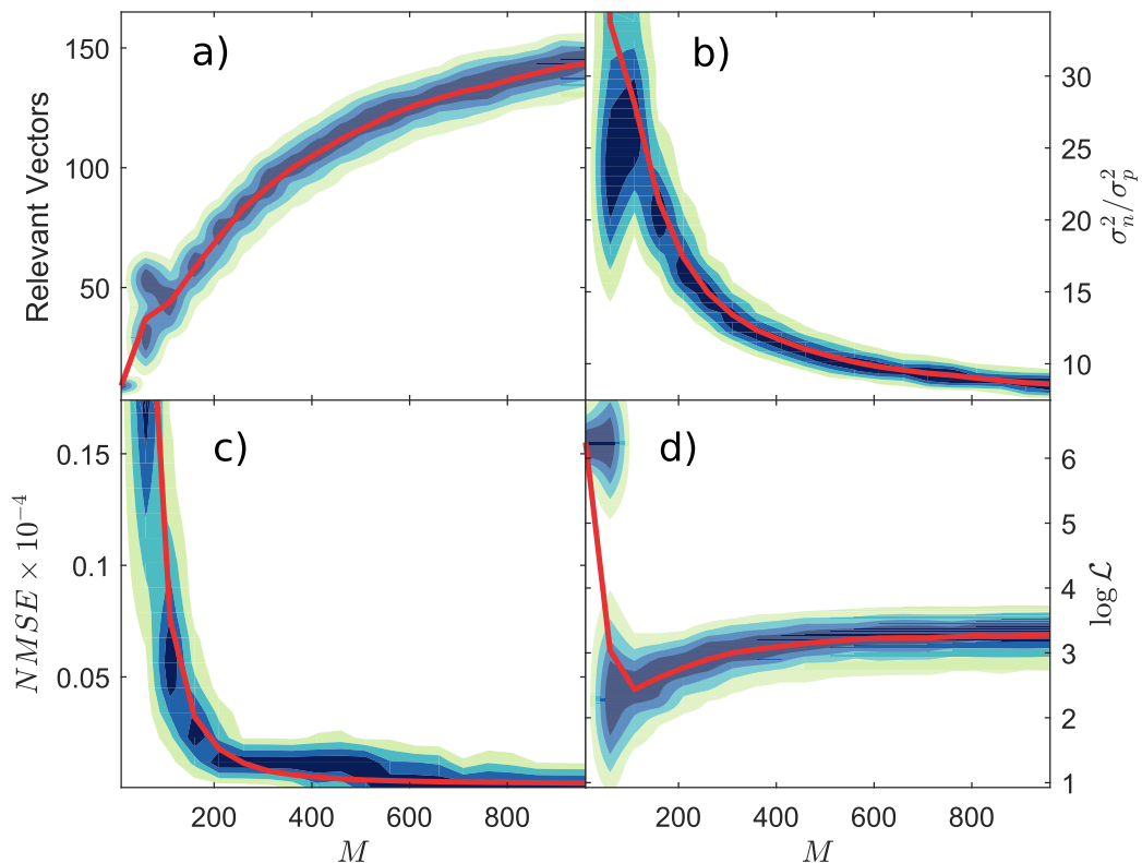
Fig. 8. Compressed dimension, M against a) number of selected relevant vectors, b) ratio of measurement noise to process variance, c) normalised mean squared error and d) log-likelihood. These metrics come from 500 randomly selected ultrasound pulses from the C-scan data of Fig. 1. The red line denotes the median, while the colour-map represents the density for the 500 draws.
