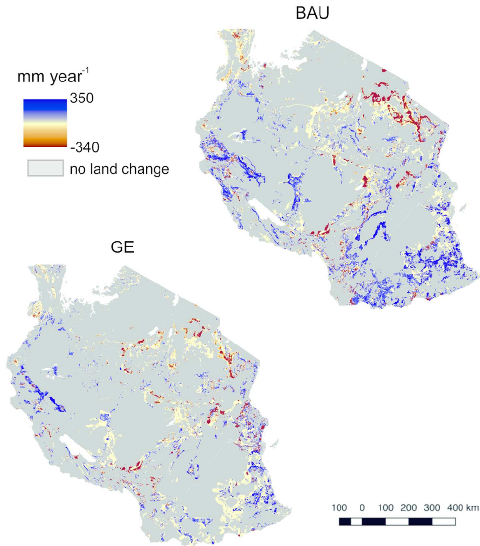
Figure 3. Changes in water yields per year (mm year -1 ) in the business as usual (BAU) and green economy (GE) scenarios across Tanzania by 2025. In both scenarios yield increment (blue shades) compared to the baseline is more frequent than yield decrease (red shades).
