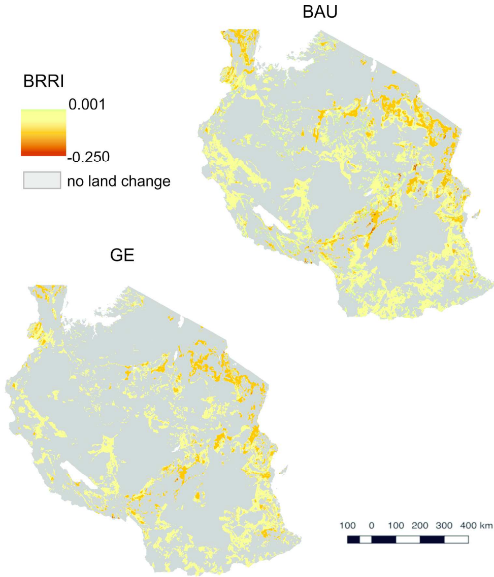
Figure 2. Changes in biodiversity richness and rarity index (BRR I) for terrestrial vertebrates in the business as usual (BAU) and green economy (GE) scenarios across Tanzania by 2025. Negative and positive changes relates to prevalent losses and gains of species suitable habitats, respectively.
