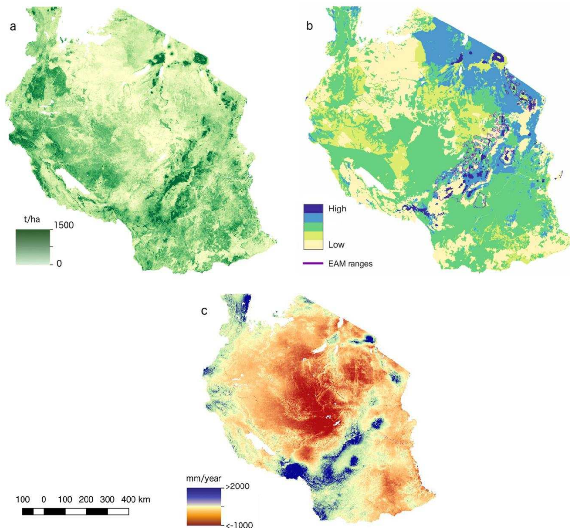
Figure S2 - Baseline maps for total carbon stock (a, \text{ton ha}^{-1} ), biodiversity richness and rarity index of terrestrial vertebrates (b, range between 0 and 0.89) and water yield (c, \text{mm year}^{-1} ) in Tanzania mainland. In b) the Eastern Arc Mountains biodiversity hotspot boundaries are represented by the purple line.
