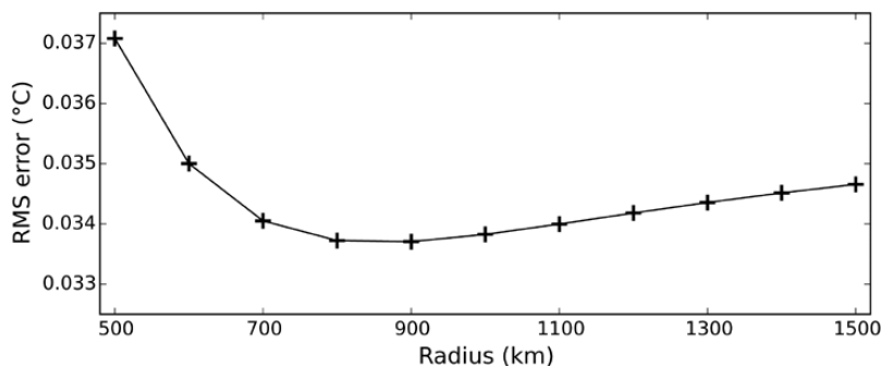
Figure 3. RMS error in global mean surface temperature estimates as a function of length-scale d_0 for the GTA1 estimator. The error is evaluated by reducing the coverage of every year of the MERRA2 reanalysis data to match the coverage of the HadCRUT4 observations for the years 1981–2010.
