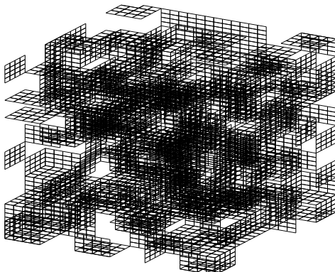
Fig. 4. 3-D representation of TLM model of random plate stirrer
