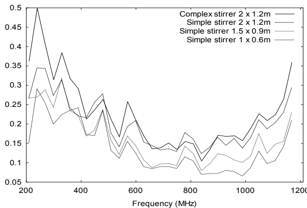
Fig. 7. The change in angle of the Poynting vector for several stirrers, cube present.
