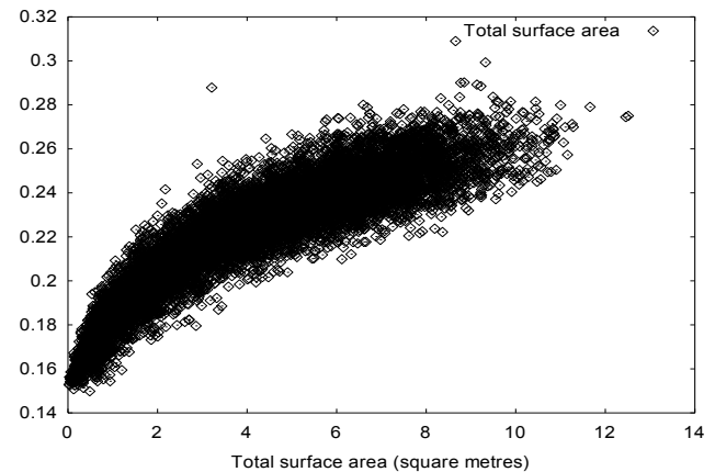
Fig. 10. Total surface area versus average change in Poynting vector
