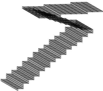
Fig. 2. 3-D representation of TLM model of complex stirrer
