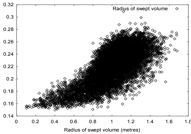
Fig. 11. Radius of swept volume versus average change in Poynting vector
