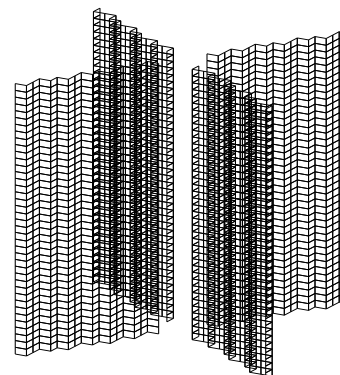
Fig. 1. 3-D representation of TLM model of simple stirrer
