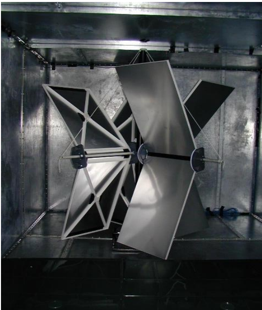
Fig. 12. The mode stirrer used in the York chamber
