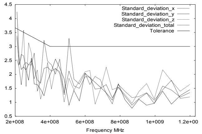
Fig. 14. Standard deviations and IEC tolerance for optimal stirrer in the York chamber
