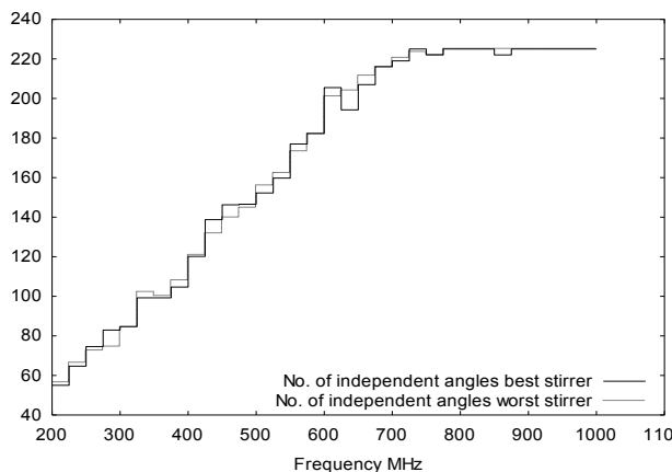
Fig. 13. The number of independent angle positions for the York stirrer
