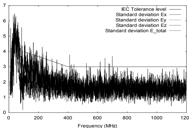
Fig. 9. Modelled standard deviation and IEC tolerance level for the best random plate stirrer
