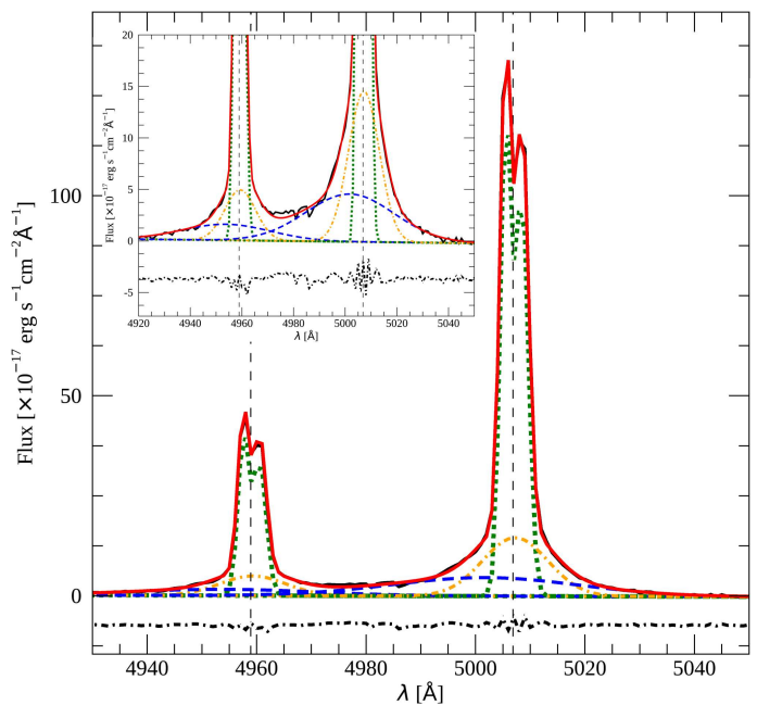
Fig. 2: [O III] \lambda\lambda 4958,5007Å doublet (black solid line) and the [O III] model (red solid line). The [O III] model includes two narrow components (1N and 2N component, green dotted line), one intermediate component (I component, yellow dot-dashed line), and one very broad component (VB component, blue dashed line). The residuals of the fit are normalized and plotted below the spectrum (black dot-dashed line). The vertical dashed line marks the restframe wavelength of the emission lines. The inset in the top left part of the plot shows a zoom-in of the I and VB components.
