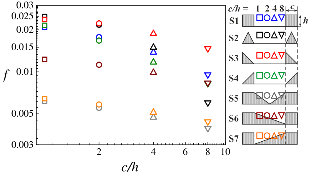
Figure 6: Darcy-Weisbach friction factor as a function of aspect ratio for flows over different roughness elements.
