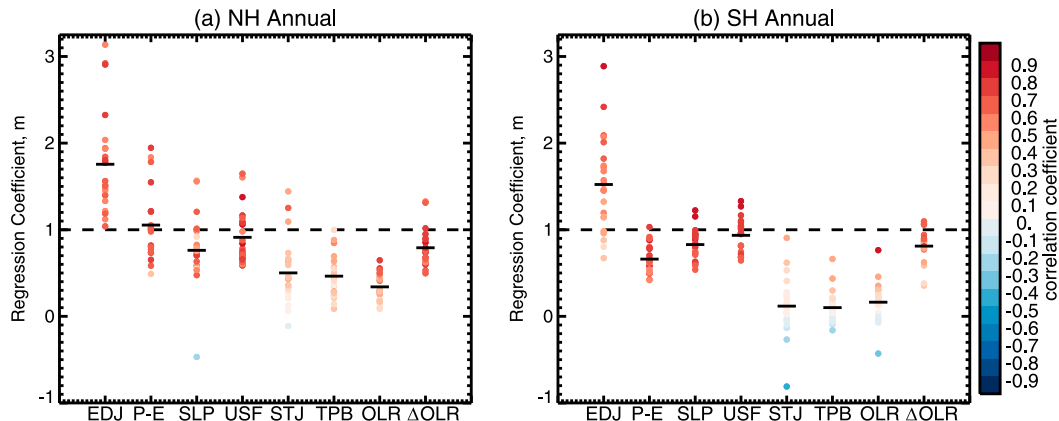
FIG. 6. Regression coefficients of metrics with PSI for annual-mean fields, for the (a) NH and (b) SH from the CMIP5 PI experiment. Symbols show individual models, the horizontal bar shows multimodel mean, and the color of the symbols denotes the correlation coefficient r .
