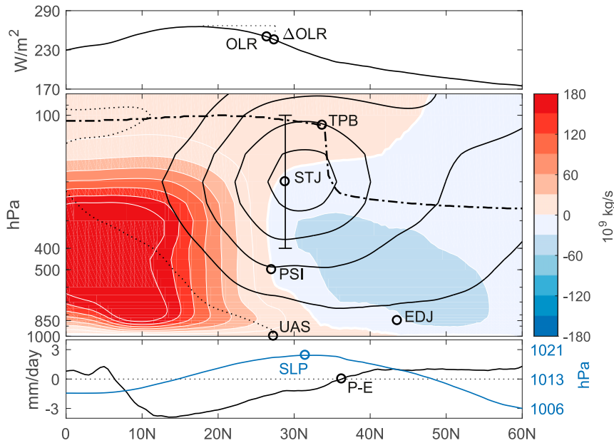
FIG. 1. Schematic illustrating the NH atmospheric circulation and structure, with the location of tropical width metrics listed in Table 2 marked with symbols: (top) outgoing longwave radiation; (middle) zonal winds (black contours; zero: dotted curve), meridional streamfunction (color shading), and tropopause (dot-dashed curve); and (bottom) sea level pressure (blue) and P-E (black). Based on MERRA-2 for February 2002.
