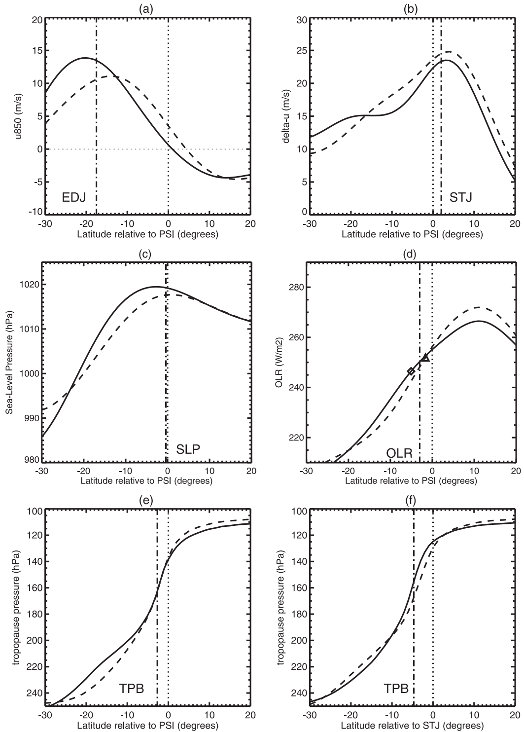
FIG. 7. Latitudinal variation of zonal-mean fields associated with a poleward (solid curve) or equatorward (dashed curve) shift of PSI from its climatological position, for the SH annual mean, for (a) u850, (b) \Delta u , (c) sea level pressure, (d) outgoing longwave radiation, and (e) tropopause pressure. (f) As in (e), but for shift of STJ. Regression analysis is performed for each individual model, and plots show multimodel mean. For (a)–(d) the curves correspond to 2° shifts in PSI from the climatological position, whereas in (e) and (f) they correspond to 10° shifts. Fields are plotted against the latitude relative to the climatological location of the PSI metric [or STJ for (f)] (vertical dotted line), and the vertical dot-dashed line is the climatological location of the metric. The triangle and diamond in (d) correspond to the mean location of the \Delta OLR metric for an equatorward and poleward shift of PSI, respectively.
