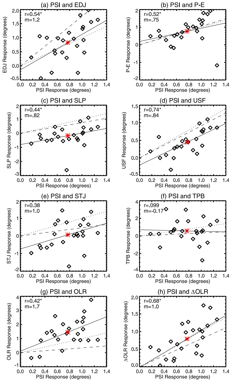
FIG. 9. As in Fig. 8, but for the NH annual mean.
