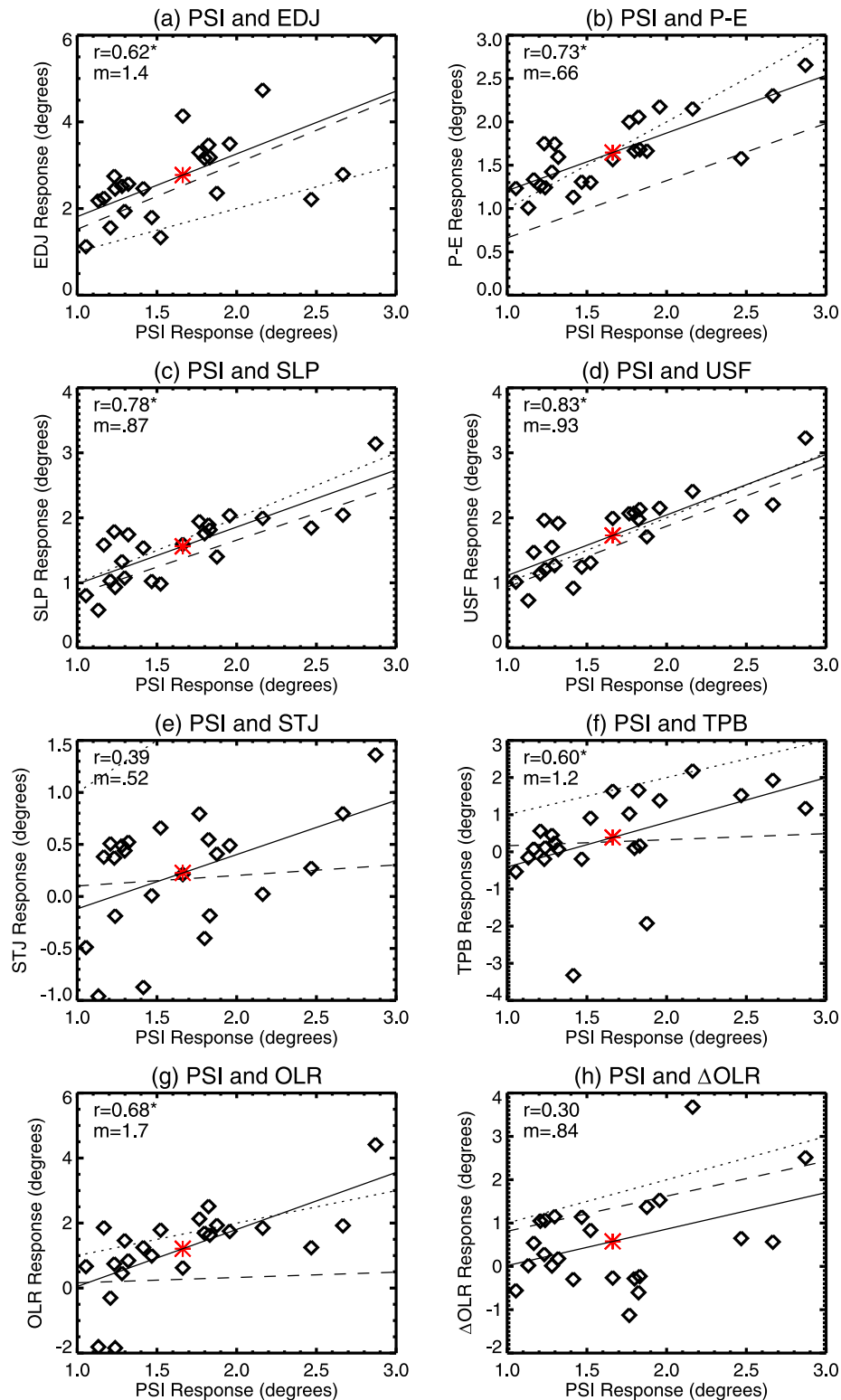
FIG. 8. Relationships between the response of SH annual mean metrics to 4\times\text{CO}_2 with that of PSI. Each diamond is a different model, and red asterisks are the multimodel means. The solid lines are the linear fits to 23 models, the dashed lines have slope equal to the regression coefficient m from the interannual regression analysis (Fig. 6), and the dotted lines indicate the 1:1 lines. Correlation coefficient r (asterisk indicates significance at 95% confidence level) and slope m are given in the legend.
