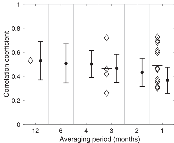
FIG. 4. Multimodel-mean correlation coefficients between PSI and EDJ in the SH for PI simulations, for interannual correlations between the annual-mean, seasonal-mean, or monthly mean metrics (diamonds at 12 months, 3 months, and 1 month), and correlations from deseasonalized monthly mean time series filtered by 1–12 months (black dots for multimodel mean and whiskers for one standard deviation). Horizontal bars show the average of interannual correlations from the seasonal-mean or monthly mean metrics (i.e., average of diamonds). Lowest correlations occur for winter months or season and highest for summer months or season.
