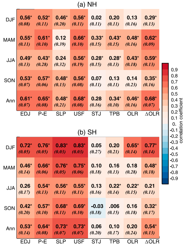
FIG. 3. CMIP5 PI multimodel-mean (and standard deviation in italics) of correlation between different metrics and PSI, for the (a) NH and (b) SH. Results are shown for each season, and for metrics based on annual-mean fields in the PI simulation. An asterisk indicates that at least 20 of the 23 models analyzed have a significant correlation (at the 95% confidence level).
