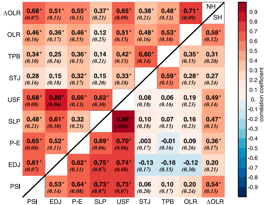
FIG. 5. Multimodel-mean (standard deviation) correlation between pairs of metrics based on annual-mean fields. Upper left is NH and lower right is SH. An asterisk indicates pairs where more than 20 of the 23 models show statistically significant correlations (at 95% confidence level).
