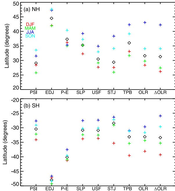
FIG. 2. Multimodel-mean location of each metric, for the annual mean (black diamonds) or for each season, DJF (red plus signs), MAM (green plus signs), JJA (blue plus signs), and SON (cyan plus signs), in the PI simulations.
