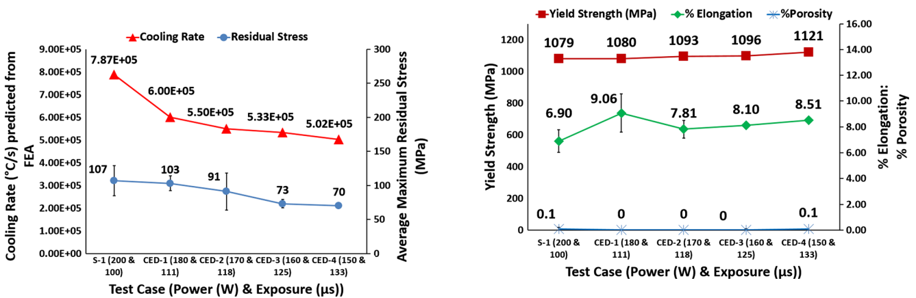
Fig. 9 Effect of varying power and exposure time combination for a constant energy density on % porosity, % elongation and yield strength
