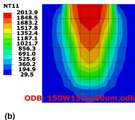
Fig. 4 Effect of varying power and exposure time combination for a constant energy density on melt-pool temperature distribution. (a) Test case S-1 (200 W power and 100 μs exposure). (b) Test case CED-4 (150 W power and 133 μs exposure)
