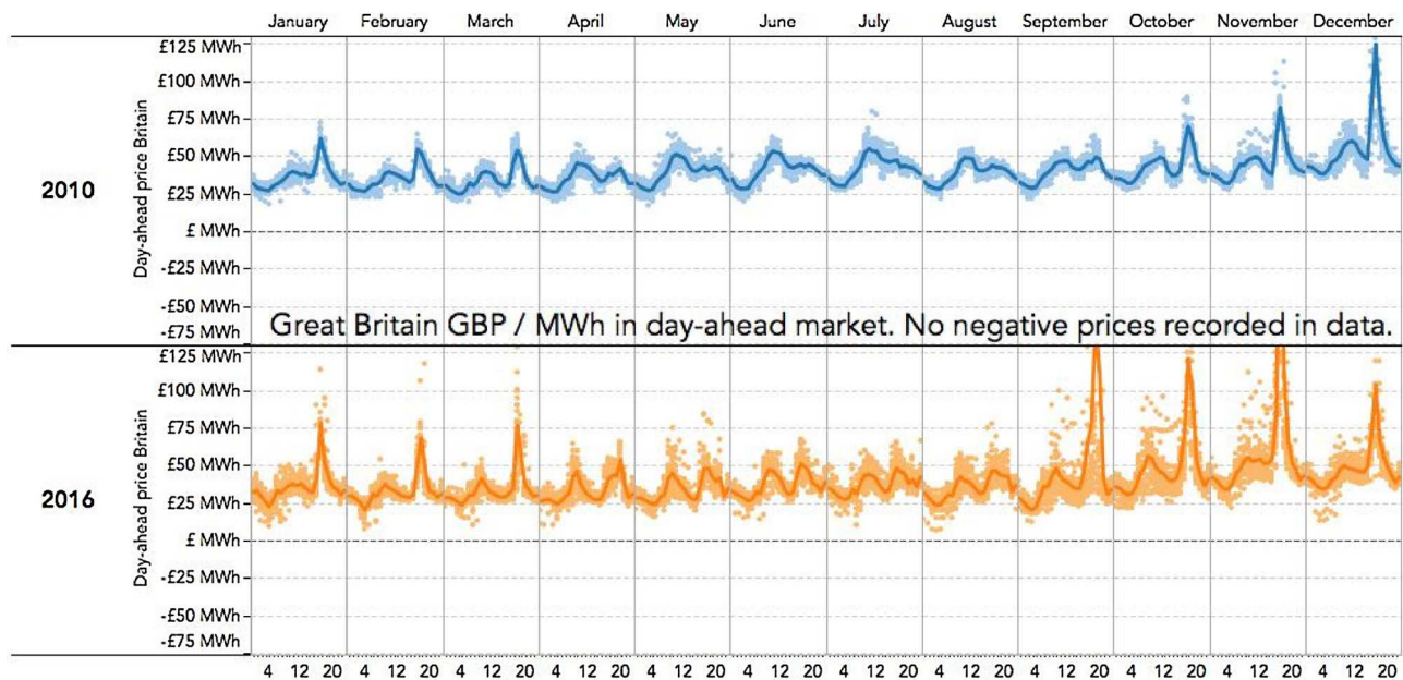
Fig. 3. The numbers on the bottom axis 4,12 and 20 refer to the hours of the day (from 1 to 24). Each cell in the Figure shows the data points for the day-ahead price per MWh, with a line showing the mean prices, for each hour and each month for 2010 (blue) and 2016 (orange). Source [27] prices for Britain. (For interpretation of the references to colour in this figure legend, the reader is referred to the web version of this article.)
