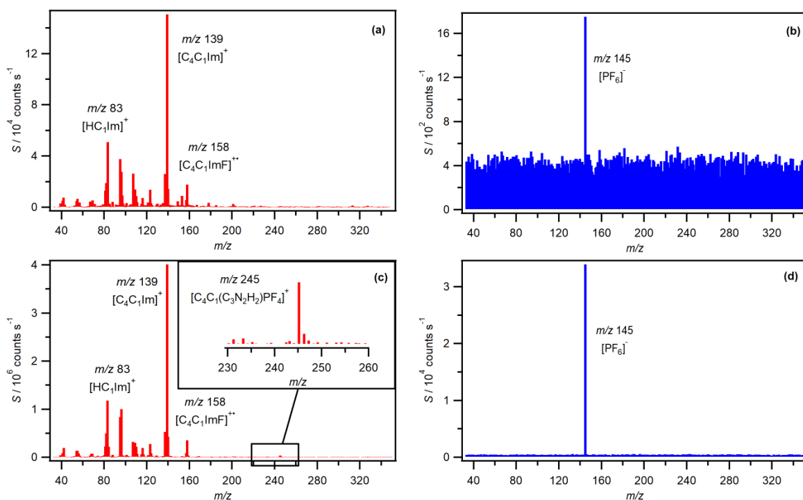
Figure 7 Mass spectrum intensity versus m/z for [C_4C_1Im][PF_6] : (a) positive mode at 493 K, (b) negative mode at 503 K, (c) positive mode at 623 K, (d) negative mode at 623 K.
