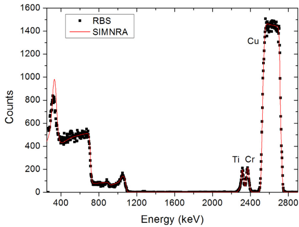
Fig. 2. RBS spectrum of the substrate measured using a 3.5 MeV ^4\text{He}^{++} beam. The points correspond to the experimental data and the line to the SIMNRA simulation [12]. From higher to lower energy the peaks correspond to Cu, Cr, Ti and kapton elements; see text for details.
