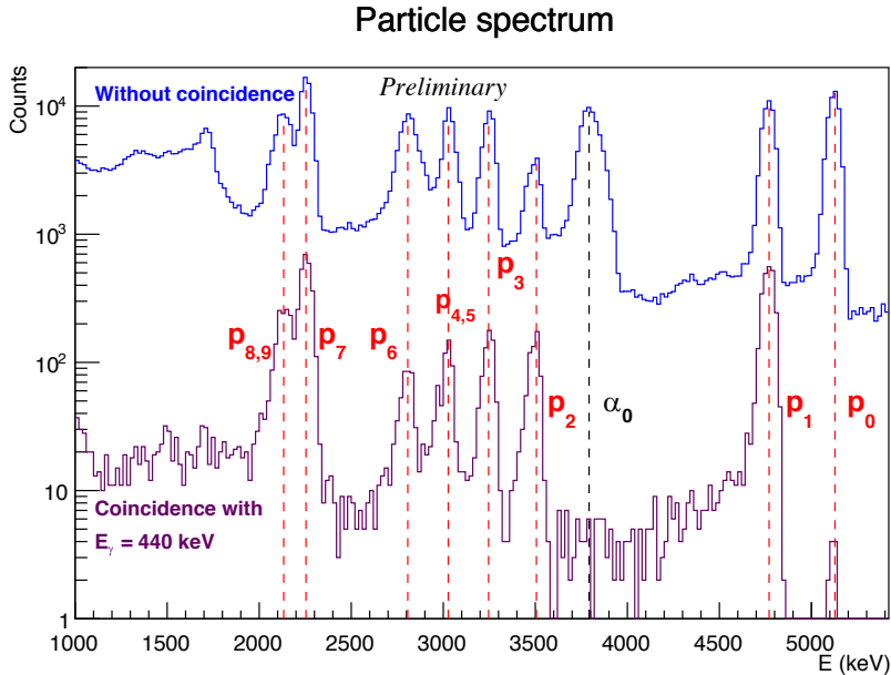
Fig. 2. (color online) Blue: ^{12}\text{C}+^{12}\text{C} fusion reaction particle spectrum measured in the STELLA project at E_{\text{lab}} = 11 MeV. Purple: same spectrum in coincidence with the 5/2^+ \rightarrow 3/2^+ transition of ^{23}\text{Na} , from ^{23}\text{Na}+p channel.
