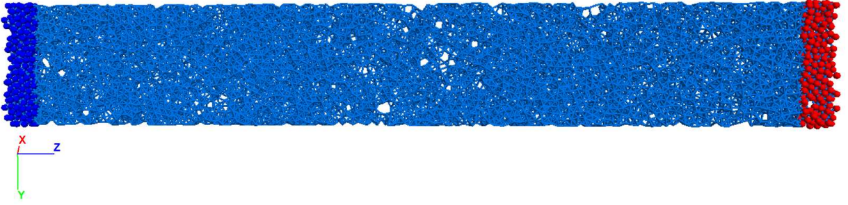
Figure 5: 3D discrete lattice model with a contact radius of 1.8
