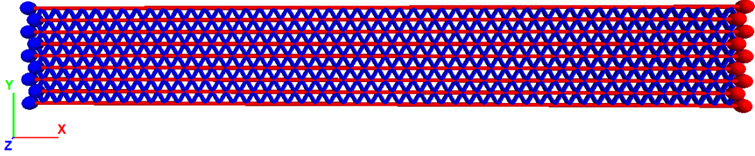
Figure 12: Extended 2D Hexagonal DEM model of 0^\circ ply composite lamina
