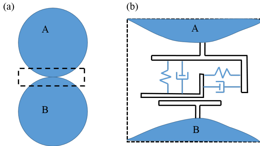
Figure 1: Representation of a contact between two particle elements in 3D DEM: (a) two particles in contact and (b) the physical elements of the contact
