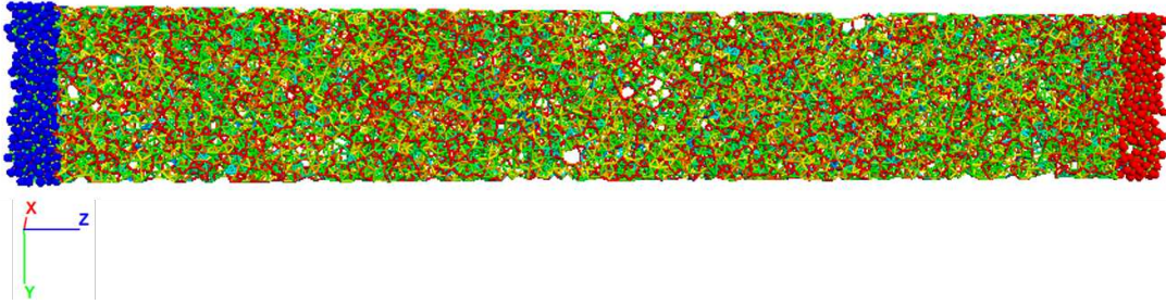
Figure 10: 3D discrete lattice DEM model of 0^\circ ply composite lamina
