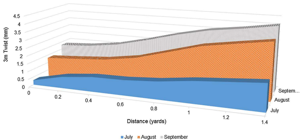
Fig. 10. Evolution of 3 m twist rail track quality parameter for a track section.
