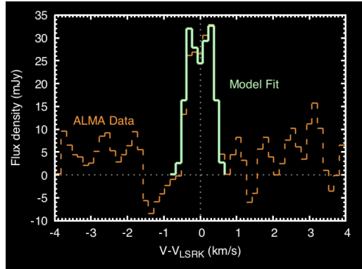
Figure 1. Methanol line profile from TW Hya extracted from the stacked channel maps within the 3\sigma contour of the 317 GHz continuum emission (orange dashed line) compared with the model fit line profile (green solid line). Figure adapted from Walsh et al. (2016).
