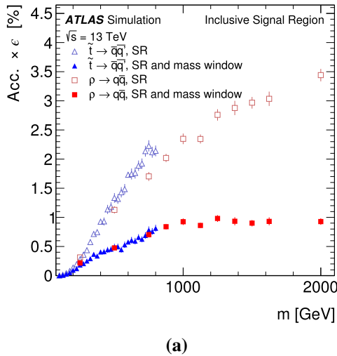
Fig. 4 The acceptance times efficiency ( \text{Acc.} \times \epsilon ) of the a inclusive and b b -tagged signal region selection as a function of the resonance mass, m , before and after the mass window requirements are applied.
