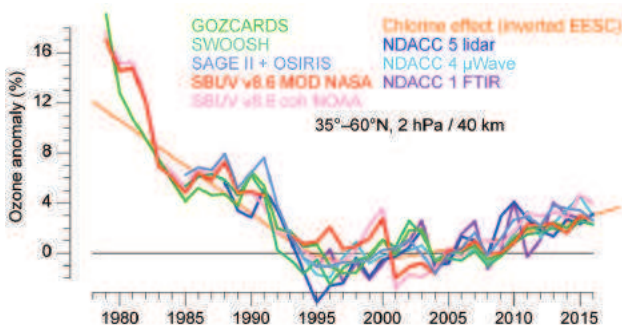
FIG. 2.52. Annual mean upper stratospheric ozone anomalies at 2 hPa ( \sim 40 km) in the zonal band 35^{\circ} – 60^{\circ} N. Data are from the merged SAGE II/OSIRIS (Bourassa et al. 2014), GOZCARDS (Froidevaux et al. 2015), SWOOSH (Davis et al. 2016b), the BUV/SBUV/SBUV2 v8.6 merged products from NASA (Frith et al. 2014) and NOAA (Wild et al. 2016) as well as averages from five lidars, four microwave radiometers, and one FTIR measuring from the ground (Steinbrecht et al. 2009; Vigouroux et al. 2015). The anomaly basis for all time series is the 1998–2008 average of annual means. The thin orange curve represents EESC, inverted and scaled to reflect the expected ozone variations due to changes in stratospheric halogens. Data points for 2016 are still preliminary as of early 2017.
