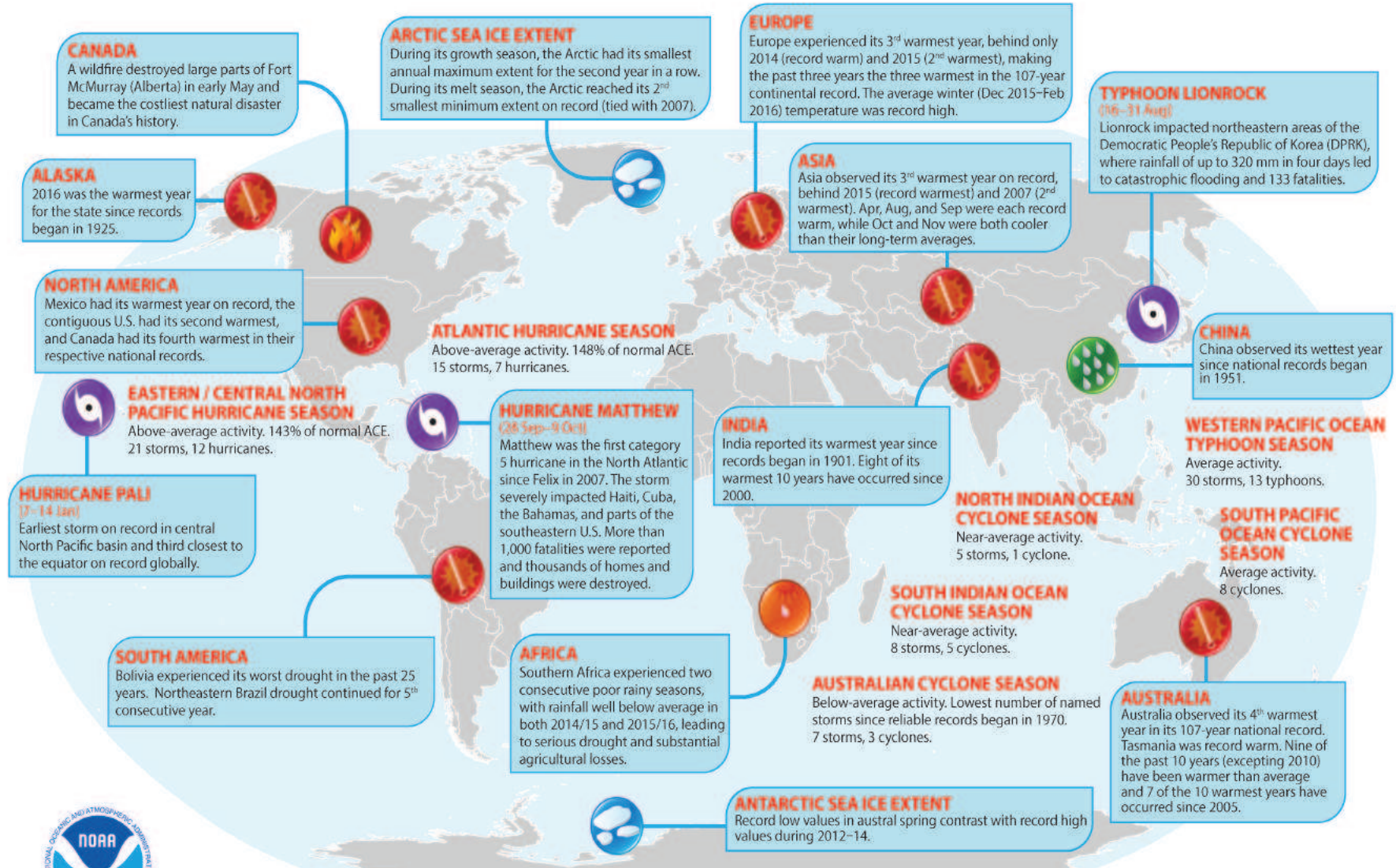
FIG. I.1. Geographical distribution of selected notable climate anomalies and events in 2016.
