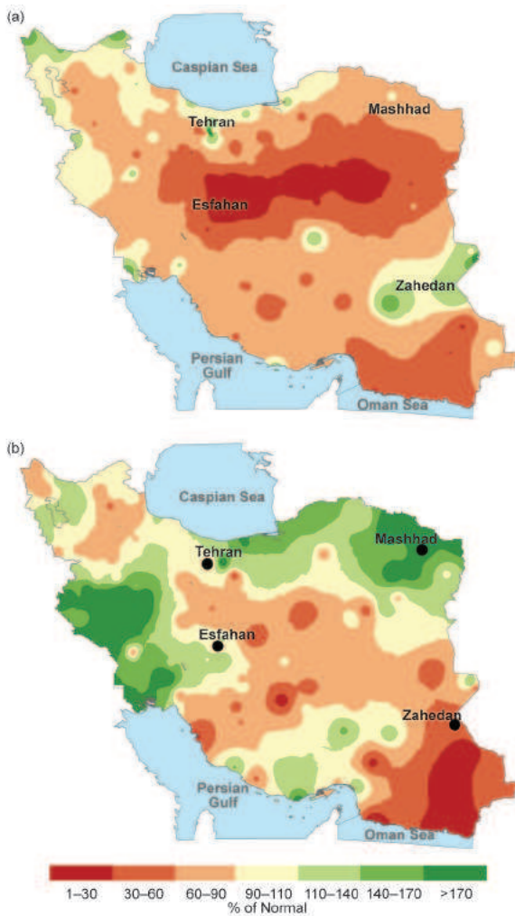
FIG. 7.52. Observed 2016 precipitation (% of mean; 1996–2015 base period) for Iran for (a) winter and (b) spring. (Source: I. R. of Iran Meteorological Organization.)
