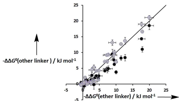
Fig. 8 Total free energy change due to intra-molecular H-bonding for ligands with an ether linker, \Delta\Delta G^0(\text{ether linker}) , compared with data for the corresponding ligands with an ester linker (black) and aromatic linker (grey), \Delta\Delta G^0(\text{other linker}) . The line corresponds to \Delta\Delta G^0(\text{other linker}) = \Delta\Delta G^0(\text{ether linker}) .
