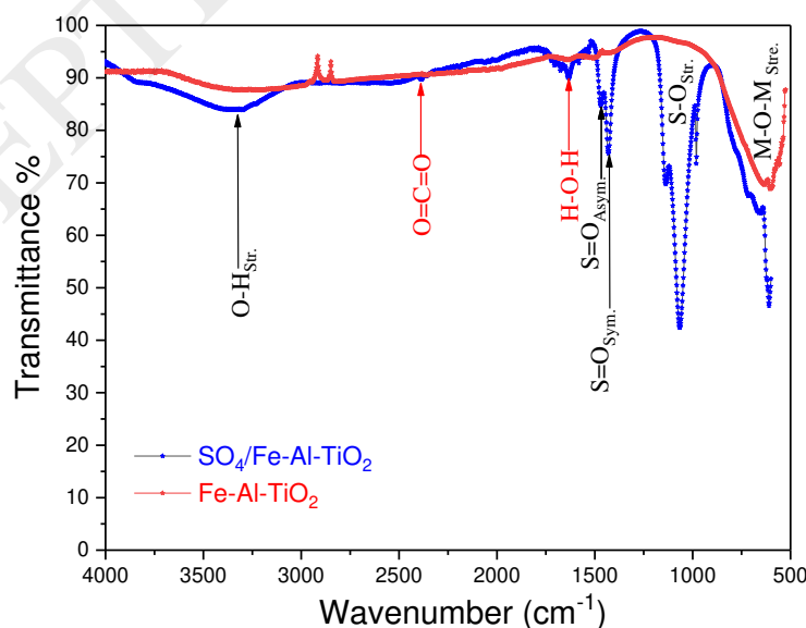
Figure 5. FTIR spectra of Fe-Al-TiO 2 and SO 4 /Fe-Al-TiO 2
