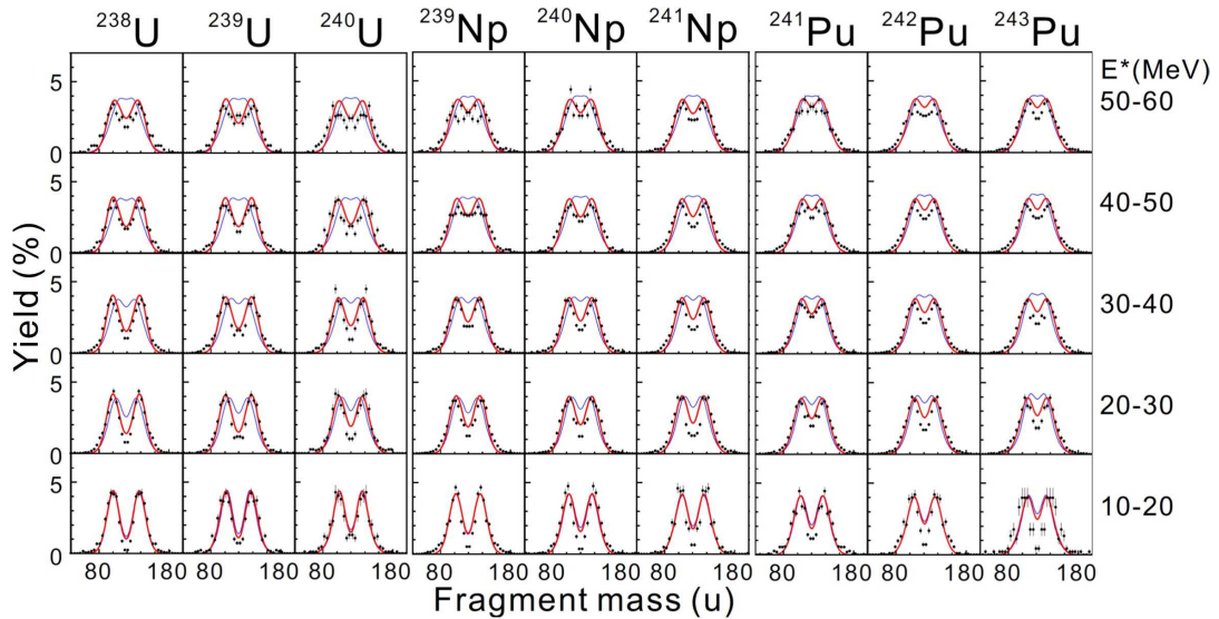
Figure 5. Experimental FFMDs (points with error bars) of the U, Np and Pu isotopes and their dependence on the excitation energy in the range of E^* = 10-60 MeV. The experimental FFMDs are compared with the Langevin calculations without (blue curves) and with (red curves) the inclusion of the multi-chance fission (see text).
