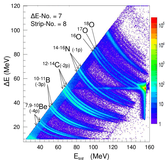
Figure 2. \Delta E - E_{\text{tot}} spectrum for ejectiles measured by one pair of the \Delta E -E detectors obtained in the ^{18}\text{O}+^{232}\text{Th} reaction [7]. The curves corresponding to different ejectiles are marked with the respective isotopes. The scattered ^{18}\text{O} is also seen in the plot.
