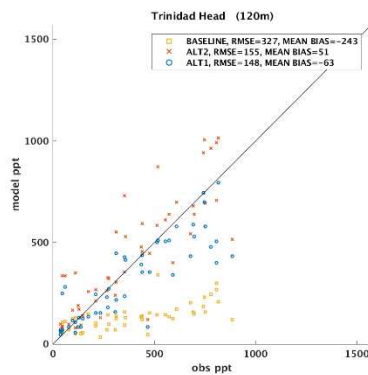
Figure S6: Comparison of modeled and observed ethane and propane for non-Arctic U.S and Canadian station for the year 2011. All stations are reported to GAW-WDCG under NOAA/INSTAAR, and were accessed May 2017.
