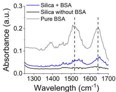
Figure 8: FTIR analysis on bioinspired silica with and without active species encapsulation. Spectra showed: black line: bioinspired silica, gray line: pure BSA, blue line: bioinspired silica loaded with BSA. Vertical dashed lines indicate characteristic amide bands.
