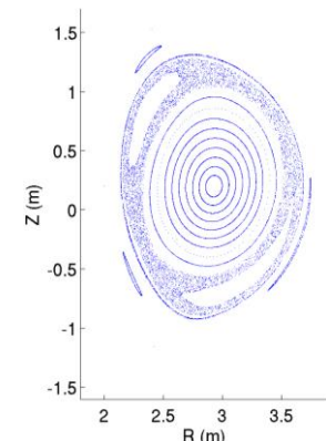
Figure 5: Current quench
