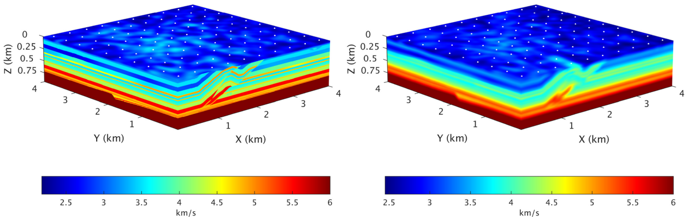
Figure 20. P -wave velocity model of the 3-D overthrust model (Aminzadeh et al. 1997). White dots show the surface projection of the monitoring arrays. Left: original velocity model used for full wavefield modelling. Right: smoothed velocity model used for source location.
