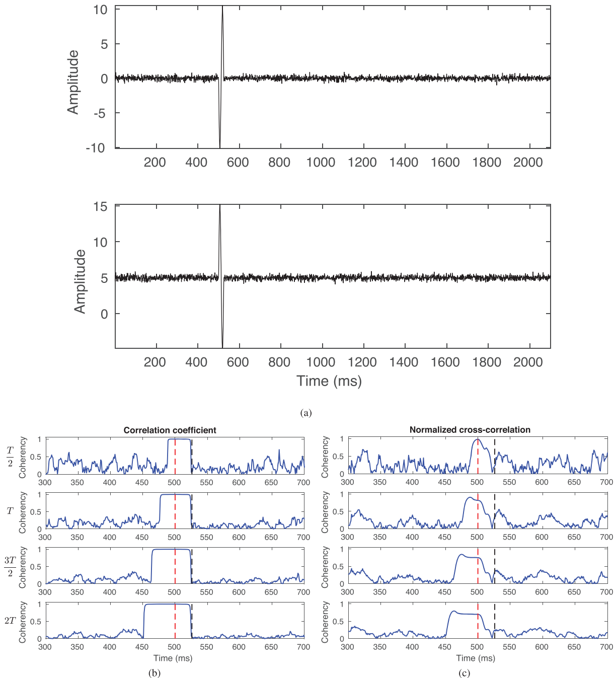
Figure 3. Coherency of two sinusoidal signals with random noise obtained by a sliding time window of different size. The period ( T ) of the sinusoidal signal is 25 ms. The top row of figures (b) and (c) shows the case with a time window of 13 ms ( T/2 ), the second row with a time window of 25 ms ( T ), the third row with a time window of 38 ms ( 3T/2 ), the bottom row with a time window of 50 ms ( 2T ). The red dashed line exhibits the origin time of the sinusoidal signal at 500 ms. The black dashed line exhibits the end time of the sinusoidal signal at 526 ms. (a) The two sinusoidal signals with random noise. The signal-to-noise ratio is 10. (b) The coherency obtained by the Pearson correlation coefficient method using eq. (3). (c) The coherency obtained by normalized cross-correlation method using eq. (4).
