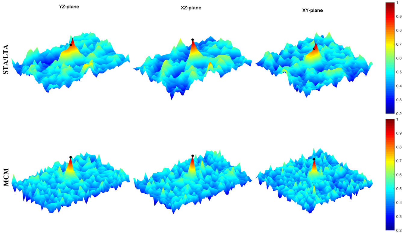
Figure 11. 3-D profiles of the migration results through the maximum migrated value of normalized stacking functions for the STA/LTA and MCM methods. Black balls show the location of the source event. The first column shows YZ profiles, second column shows XZ profiles, third column shows XY profiles. The first row shows results of the STA/LTA method, second row for MCM.
