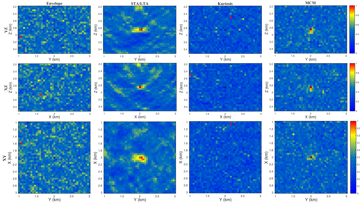
Figure 10. Profiles of the migration results through the normalized stacking functions at the stacking maximum for the four migration methods. NSR = 6. For better comparison of different migration results, all the stacking functions have been linearly normalized to the range between 0 and 1. Black hexagrams in the middle of the target area represent the true source location. The first column shows results of envelope, second column for STA/LTA, third column for kurtosis, fourth column for MCM. The first row shows YZ (vertical) profiles, second row shows XZ (vertical) profiles, third row shows XY (horizontal) profiles.
