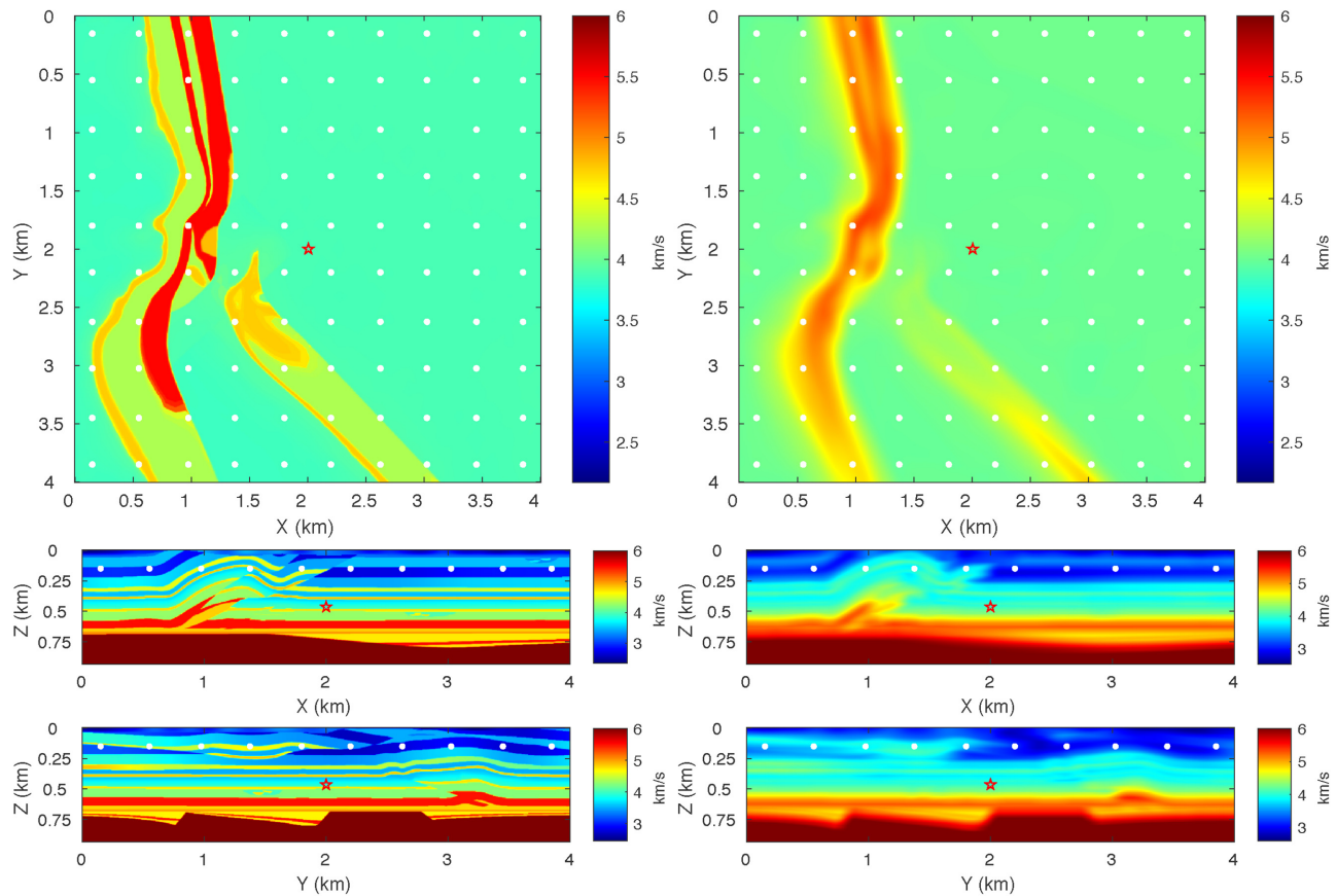
Figure 21. P -wave velocity profiles of the 3-D overthrust model through the source point. Red star shows the location of the source and white dots show the projection of receivers. First row: horizontal profiles at the depth of 0.46 km. Second row: vertical profiles at 1.995 km in the Y direction. Third row: vertical profiles at 1.995 km in the X direction. Left: original velocity model used for full wavefield modelling. Right: smoothed velocity model used for source location.
