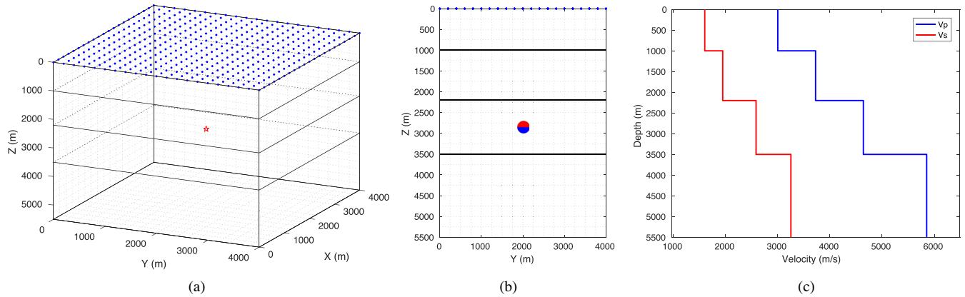
Figure 8. The velocity model and receiver geometry for the microseismic monitoring. (a) Layered model showing the velocity and surface array. The red star represents the vertical dip-slip source, blue points represent the surface receivers. 441 receivers are uniformly distributed on the free surface with 21 receiver lines in X direction, 21 receiver lines in Y direction and a lateral interval of 200 m. (b) Vertical profile of the layered model with a beach ball showing the moment tensor source. (c) P - and S -wave velocities used for the migration.
