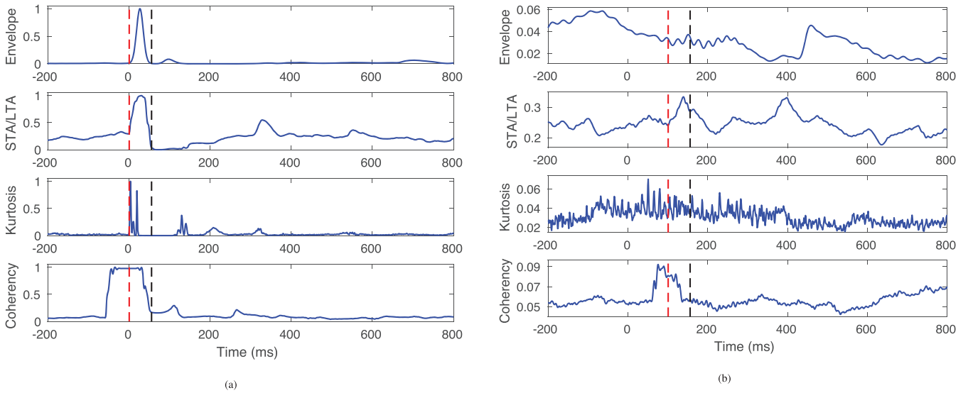
Figure 17. The stacking functions at the true source locations of (a) event 1 and (b) event 2 for the four methods. The red and black dashed line shows the origin time and end time of the events 1 and 2, respectively.
