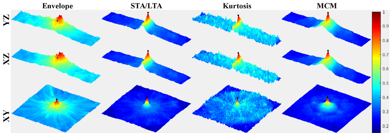
Figure 23. 3-D profiles of the migration results using the smoothed overthrust velocity model for the four methods. The profiles are obtained by projecting the maximum stacking values along the time domain and the corresponding directions (i.e. for YZ profiles, projecting along the X direction; for XZ profiles, projecting along the Y direction; for XY profiles, projecting along the Z direction). Black balls show the true position of the source event. The migrated volumes of different methods are all linearly normalized to 0–1. The first column shows results of envelope, second column for STA/LTA, third column for kurtosis, fourth column for MCM. The first row shows YZ (vertical) 3-D profiles, second row shows XZ (vertical) 3-D profiles, third row shows XY (horizontal) 3-D profiles.
