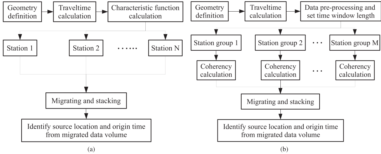
Figure 2. (a) Workflow of the traditional migration-based location method. (b) Workflow of the MCM method.
