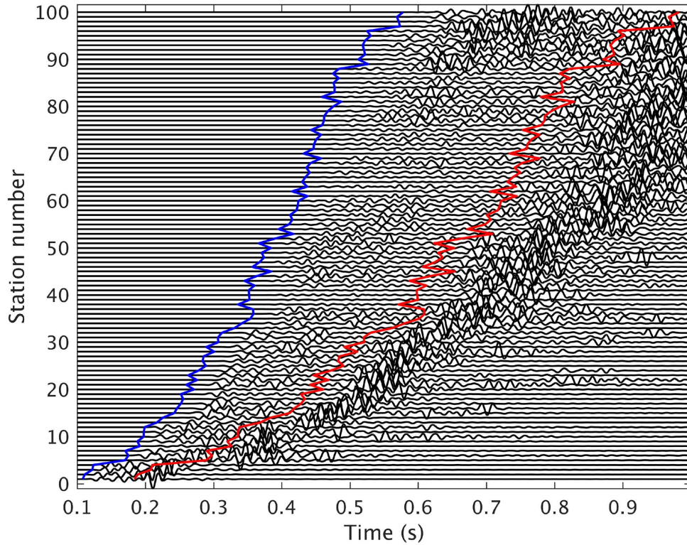
Figure 22. Record section of particle velocities in the Z direction for the 3-D overthrust model. Blue line shows the calculated arrival times for the direct P-waves and red line shows the calculated arrival times for the direct S-waves. The recorded traces are numbered and aligned vertically according to horizontal offsets. Note that the calculated arrival times of the direct P- and S-waves are not smooth (zigzagged) because of strong 3-D heterogeneity of the model.
