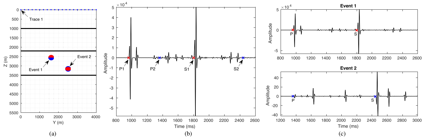
Figure 14. (a) Model profile which shows the positions of two events. Event 1 is a vertical dip-slip source and event 2 is a 45 degree dip-slip source. Beach balls are used to show the radiation pattern of the moment tensor sources. (b) The recorded seismogram in trace 1. The red crosses show the P - and S -wave arrivals of event 1. The blue crosses show the P - and S -wave arrivals of event 2. (c) Separate wavefields of events 1 and 2.
