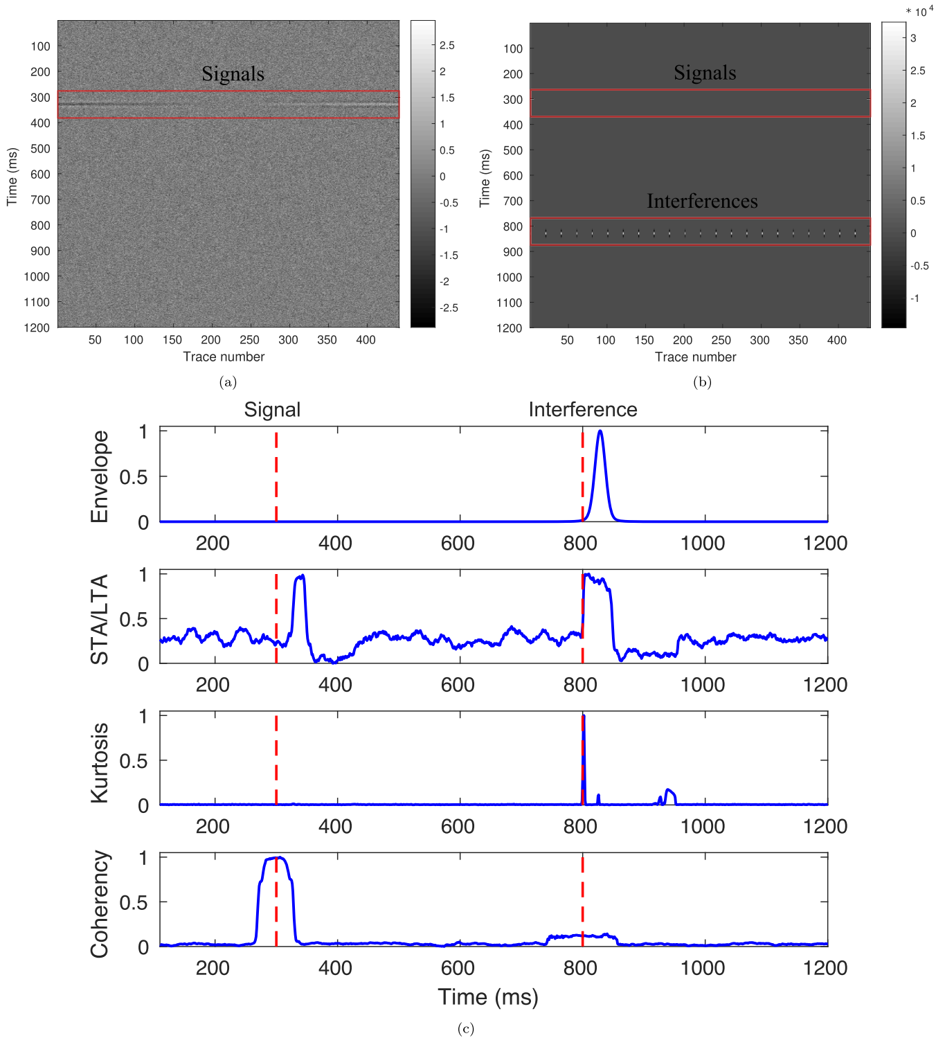
Figure 13. (a) The time aligned traces with NSR = 3 . The origin time for the weak signals to be detected is 300 ms. (b) The time aligned traces after adding strong coherent interference signals into 23 of the traces in (a). The amplitude of the interference signals is 32 768 times the amplitude of the weak effective signals. After adding interferences, the effective signals are invisible because of the enormous amplitude differences between the signals and the interferences. The origin time of the interference signals is 800 ms. Signals and interferences are annotated in the figure, respectively. (c) Stacking functions of the four different methods with red dashed lines showing the origin times of the weak signals and interference signals.
