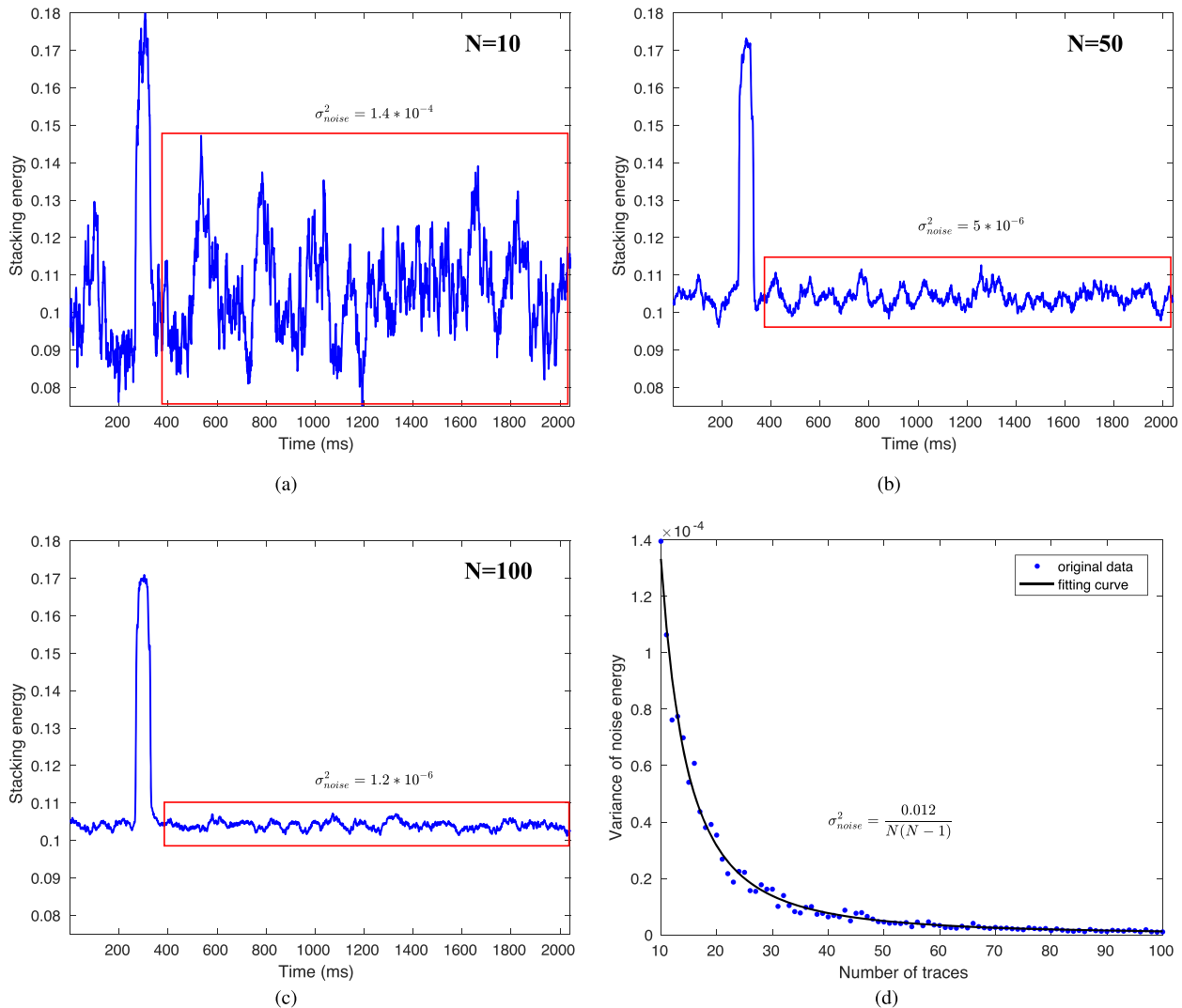
Figure 7. Stacking functions at the source position when the trace number ( N ) is (a) 10, (b) 50 and (c) 100 for the MCM method. (d) Variation of the variance of noise energy with different trace numbers at the source position for the MCM method. The results are obtained through the Monte Carlo simulation. Blue points represent the calculated variance of noise energy, and the black line shows the fit to the variance data points. The fitting formula is also shown in the figure. The NSR is 4 for all the figures.
