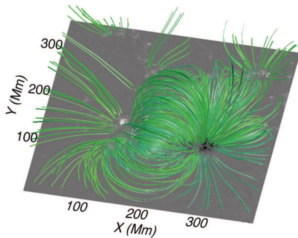
Figure 9. Extrapolated magnetic field lines (green lines) overlaid on the photospheric B_z map from HMI. This corresponds to ROSA data taken on 2011 December 10 shown in the main text, with the center of the image corresponding to the pore under analysis (see lowest image in the stack in Figure 6 of the main text). The box extends to around 110 Mm above the active region. Analyzing the free energies from these extrapolations suggests that reconnection phenomena cannot be responsible for the power enhancement at the pore boundary for our surface mode observations in the filtered data shown in the main text. Therefore, the power enhancements must be the result of wave phenomena observed in the data set.
