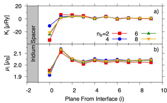
Figure 2. (a) Plane-by-plane first order uniaxial anisotropy constant, K_i and (b) magnetic moments, as a function of distance from the Ir interface. The data presented is for n_{Ir} = 2, 4, 6 and 8 planes of Ir (red, blue, green and gold respectively) as shown schematically in Fig. 11 (see methods).
