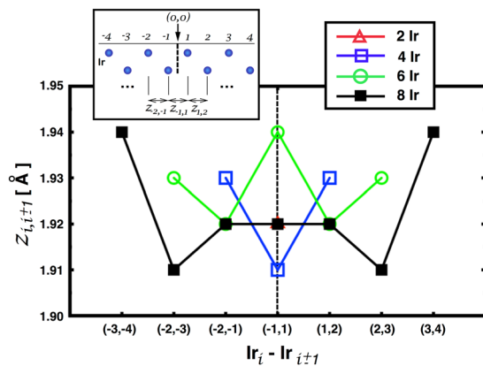
Figure 1. Out-of-plane distances between different Ir planes for ... Fe/ n_{Ir} Ir/Fe ... [ n_{Ir} = 2, 4, 6, 8] geometries. The center of each configuration has been shifted to the vertical dashed line that represents the central out-of-plane distance for any configuration. The x -axis values depict each Ir layer pair, i and i \pm 1 .
