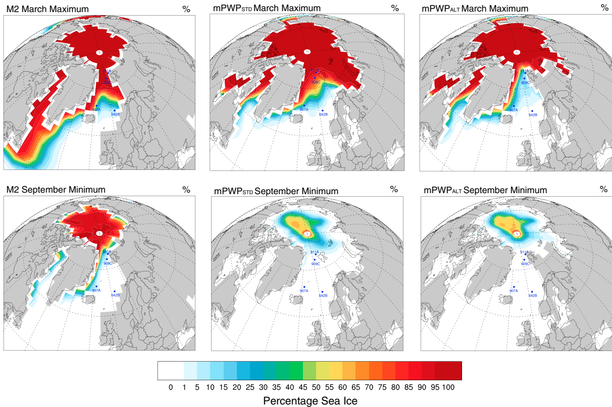
Figure 3. Extent and percentage concentration of sea ice. (top row) The March maximum extent of sea ice and (bottom row) the September minimum. M2 = Marine Isotope Stage M2; mPWP STD = standard mid-Piacenzian Warm Period; mPWP ALT = mid-Piacenzian Warm Period scenario with an altered paleogeography.
