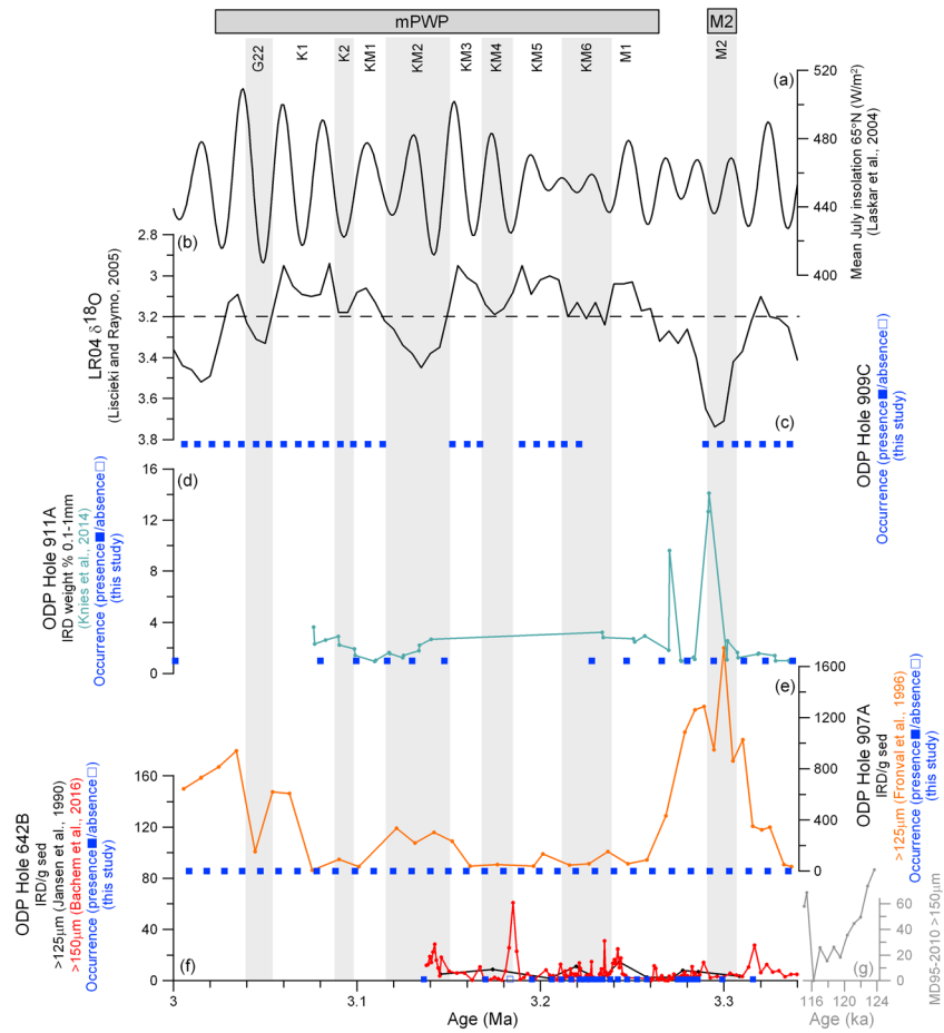
Figure 5. Ice-rafted debris (IRD) compilation for the Nordic Seas. Note different scales on the y axes. (a) July insolation at 65°N (Laskar et al., 2004). (b) LR04 stack of benthic \delta^{18}\text{O} with the current \delta^{18}\text{O} level of 3.23‰ shown as a dashed line (modified from Lisiecki & Raymo, 2005). (c) New occurrence data showing the presence (■) or absence (□) of IRD at Ocean Drilling Program (ODP) Hole 909C. For panels (d)–(f), occurrence data are also plotted in the same manner. (d) ODP Hole 911A IRD record (weight percentage of the 0.1 to 1 mm size fraction (light blue; Knies, Mattingdsdal, et al., 2014)). (e) ODP Hole 907A IRD record (number of grains >125 \mu\text{m} per gram sediment (Fronval & Jansen, 1996)). (f) ODP Hole 642B IRD record (number of grains >125 \mu\text{m} (black; Jansen et al., 1990) and >150 \mu\text{m} (red; Bachem et al., 2016, 2017)). (g) MD95-2010 IRD record covering the last interglacial (number of grains >150 \mu\text{m} (gray)). The horizontal bars denote the mid-Piacenzian Warm Period (mPWP) (Dowsett et al., 2010) and Marine Isotope Stage M2 (MIS M2) (De Schepper et al., 2009). Vertical light gray bars identify colder isotope stages (Lisiecki & Raymo, 2005).
