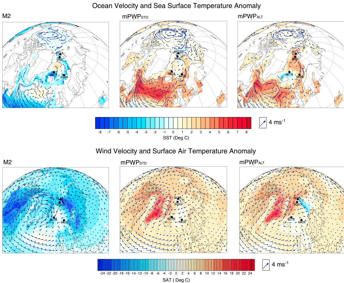
Figure 2. Climatological boundary conditions of the M2, mPWP STD , and mPWP ALT scenarios. Ocean and wind currents are the two main drivers of iceberg trajectories; however, sea surface temperatures (SST) and surface atmospheric temperature (SAT) influence the melt rate. The SST and SAT anomalies are calculated using annual mean temperatures. The wind velocity scale arrow is measured at 4 \text{ m s}^{-1} . M2 = Marine Isotope Stage M2; mPWP STD = standard mid-Piacenzian Warm Period; mPWP ALT = mid-Piacenzian Warm Period scenario with an altered paleogeography.
