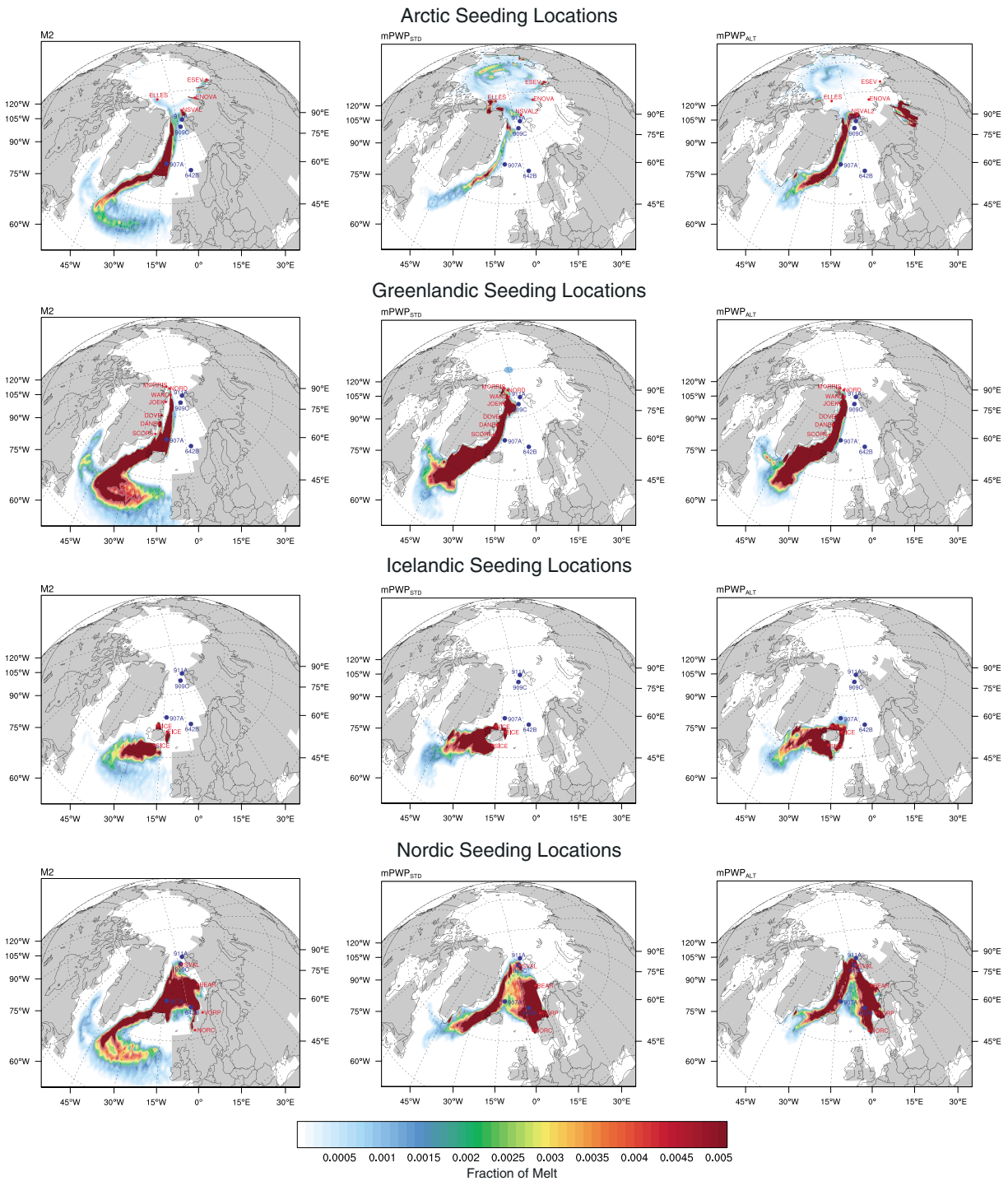
Figure 4. Iceberg trajectories for the 19 seeding locations for three different climate scenarios (M2, mPWP STD , and mPWP ALT ). M2 = Marine Isotope Stage M2; mPWP STD = standard mid-Piacenzian Warm Period; mPWP ALT = mid-Piacenzian Warm Period scenario with an altered paleogeography.
