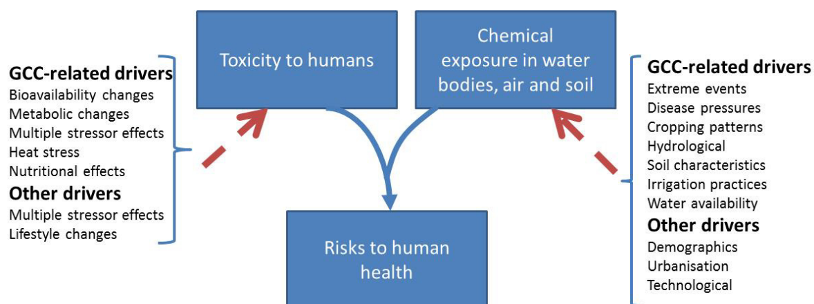
Figure 4.1 Potential global climate change (GCC) related and other drivers that will affect the risks of pollutants to human health in the UK in the future
