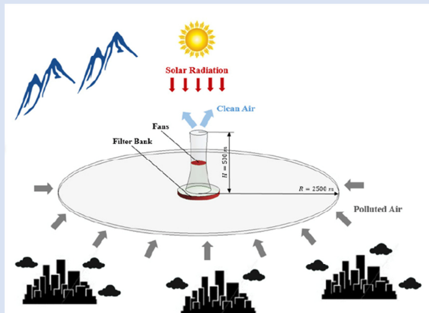
Figure A Schematic diagram of the Solar-Assisted Large-Scale Cleaning System
