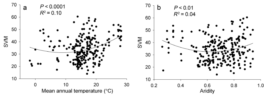
FIG. 1. Relationships between mean annual temperature and aridity (defined as 1 – aridity index [the ratio of precipitation to potential evapotranspiration]) and the variability (coefficient of variation) of soil multifunctionality (SVM). The solid lines represent the fitted regressions. R^2 shows the proportion of variance explained.
