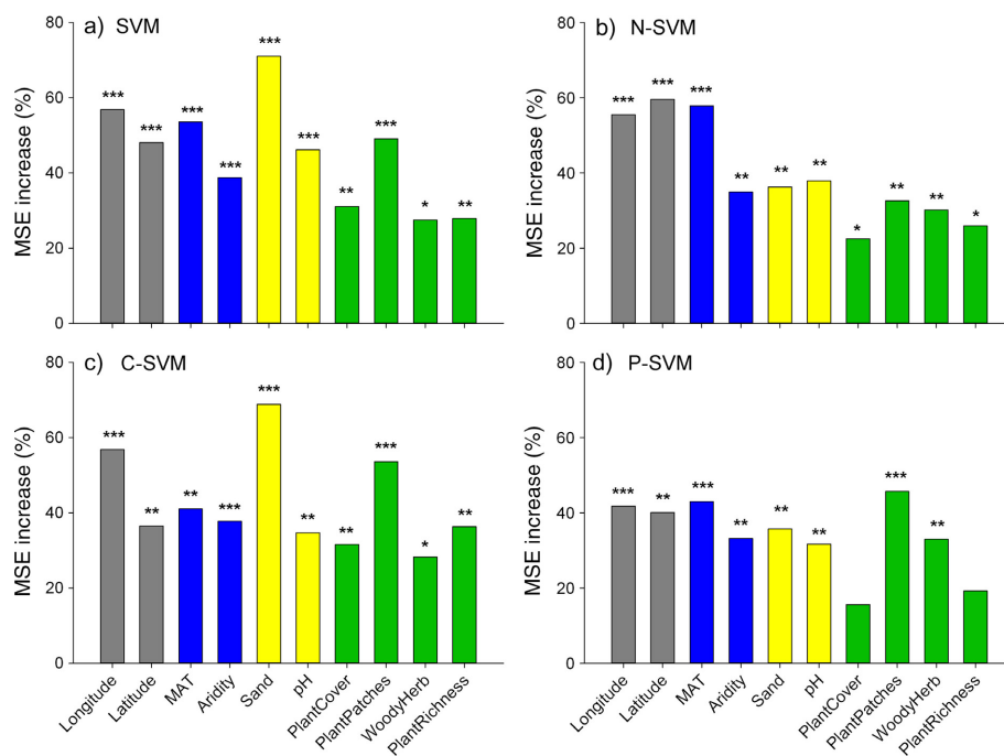
FIG. 2. Random forest mean predictor importance (increase of mean square error [MSE; %]) of biotic and abiotic drivers on the spatial variability (coefficient of variation) of (a) soil multifunctionality (SVM), (b) N-related variables (SVM-N), (c) C-related variables (SVM-C), and (d) P-related variables (P-SVM). Predictors are latitude, longitude, mean annual temperature (MAT), aridity, plant species richness (PlantRichness), plant cover (PlantCover), number of plant patches (PlantPatches), the ratio between woody and herbaceous cover (WoodyHerb), soil sand (Sand), and soil pH. Significance levels of each predictor are as follows: * P < 0.05 , ** P < 0.01 , and *** P < 0.001 .
