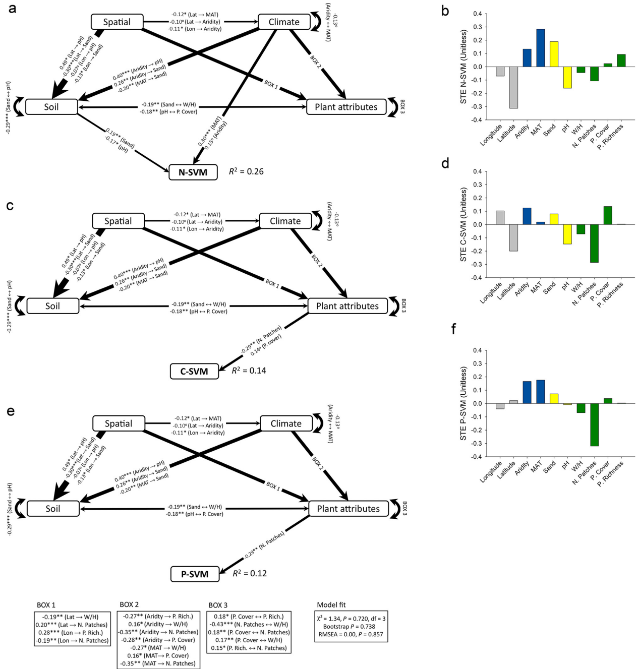
FIG. 4. Effects of mean annual temperature, aridity, soil variables (pH and sand content), biotic attributes (plant cover and richness, number of plant patches, and woody to herbaceous cover ratio [W/H]) and geographical coordinates (longitude and latitude) on the spatial variability (coefficient of variation) of the soil multifunctionality of (a) N-, (c) C-, and (e) P-related variables (N-SVM, C-SVM, and P-SVM, respectively). Numbers adjacent to arrows are standardized path coefficients, analogous to relative regression weights, and indicative of the effect size of the relationship. * P < 0.05 and ** P < 0.01 . Only significant relationships ( P < 0.05 ) are shown. Arrow widths are proportional to the strength of the relationship. Squares are observable variables. The proportion of variance explained ( R^2 ) appears alongside the response variable in the model. Goodness-of-fit statistics for each model are shown in the bottom (df = degrees of freedom; RMSEA = root mean squared error of approximation). The components within spatial geolocation, climate, soil (properties) and plant attributes are included as independent observable variables in the model, however we group them in the same box in the model for graphical simplicity. Panels b, d, and f show the standardized total effects (direct plus indirect effects derived from the structural equation models) of N-SVM, C-SVM, and P-SVM predictors, respectively.
