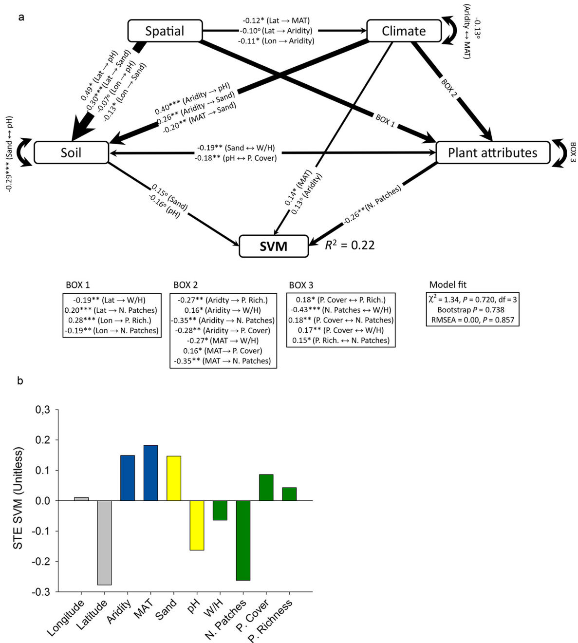
FIG. 3. (a) Effects of mean annual temperature, aridity, soil variables (pH and sand content), biotic attributes (plant cover [P. Cover] and richness [P. Rich.], number of plant patches [N. Patches], and woody to herbaceous cover ratio [W/H]), and geographical coordinates (longitude [Lon] and latitude [Lat]) on the spatial variability (coefficient of variation) of soil multifunctionality (SVM). Numbers adjacent to arrows are standardized path coefficients, analogous to relative regression weights, and indicative of the effect size of the relationship. * P < 0.05 and ** P < 0.01 . Only significant relationships ( P < 0.05 ) are shown. Arrow widths are proportional to the strength of the relationship. Squares are observable variables. The proportion of variance explained ( R^2 ) appears alongside the response variable in the model. Goodness-of-fit statistics for each model are shown in the bottom (df, degrees of freedom; RMSEA, root mean squared error of approximation). The components within spatial geolocation, climate, soil (properties) and plant attributes are included as independent observable variables in the model, however, we group them in the same box in the model for graphical simplicity. (b) Standardized total effects (direct plus indirect effects derived from the structural equation models) of SVM predictors.
