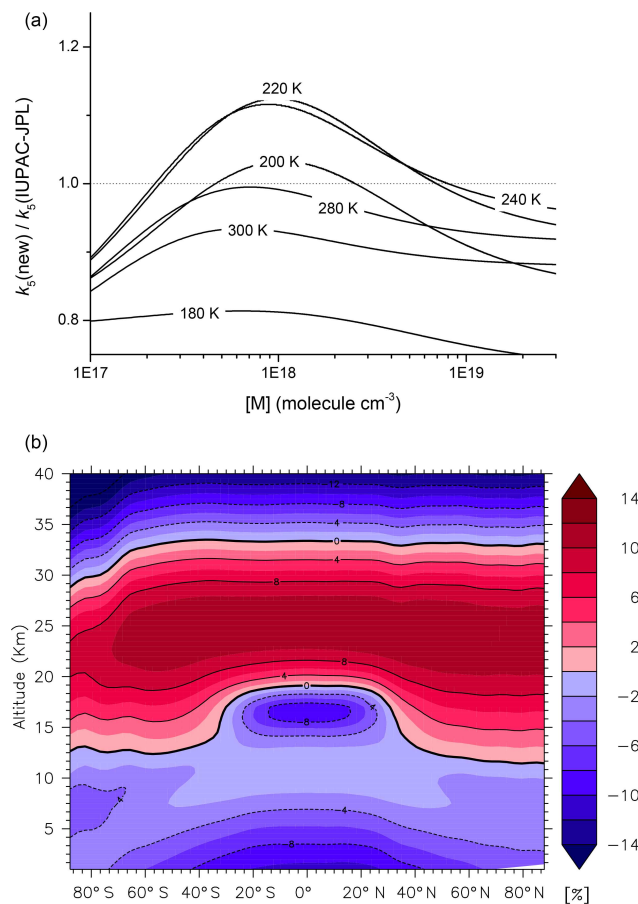
Figure 11. (a) Ratio of rate coefficients obtained by combining results from this work with selected data sets from the literature, k_5 (new), to those presently recommended by the IUPAC and JPL panels, k_5 (IUPAC-JPL). (b) Change in rate coefficient k_5 (new) compared to previous IUPAC and JPL evaluations. The percentage change was calculated using annually and zonally averaged temperatures and pressure in the EMAC model.
