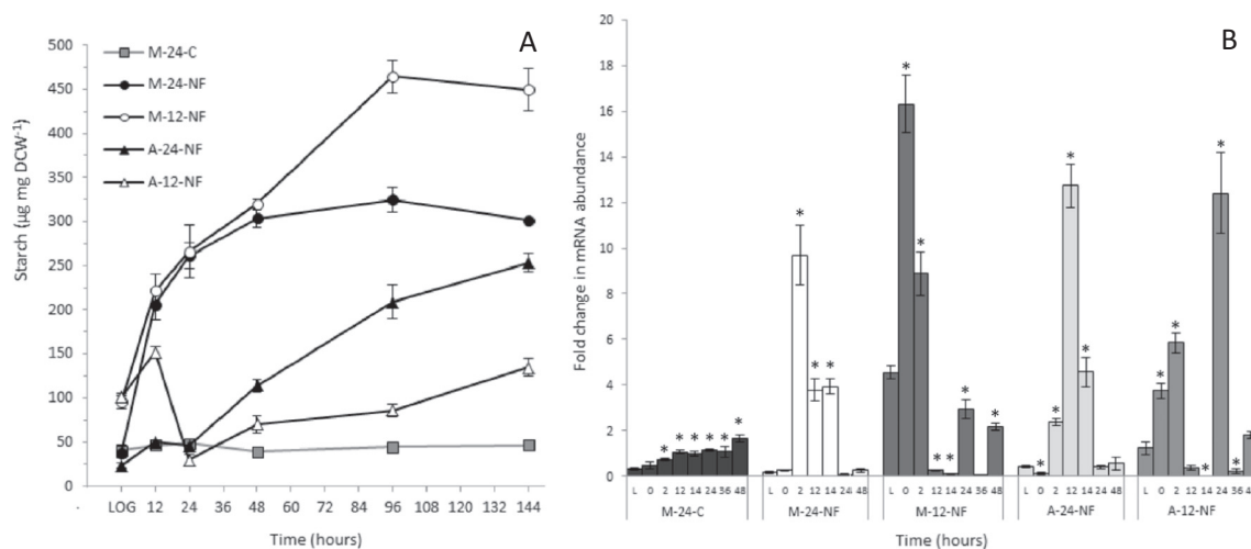
Fig. 6. A) Starch content ( \mu\text{g starch mg}^{-1}\text{DCW} ) before (LOG) and after cell resuspension in nitrogen free (NF) or replete (C) medium. B) Fold change (relative to the average gene expression of all samples across all time points and treatments) of STA2 expression, before (L) and after resuspension in nitrogen free (NF) or replete (C) medium. LOG (L), indicates sampling point at which cells were in the log (exponential) phase of growth, immediately before transfer to N deplete (–N) medium. Treatment conditions are outlined in Table 1, M-24-C, mixotrophic continuous light, C medium; M-24-NF, mixotrophic continuous light, NF medium; M-12-NF, mixotrophic diurnal light, NF medium; A-24-NF, autotrophic continuous light, NF medium; A-12-NF, autotrophic diurnal light, NF medium. Error bars represent SE ( n = 3 ), * symbols indicate significant difference from L (LOG) time point values ( t -test, p < 0.05 ). For M-12-NF and A-12-NF, L sample taken in dark period before resuspension, then 0 to 12 h light; 12 to 24 h dark; 24 to 36 h light; 36 to 48 h dark.
