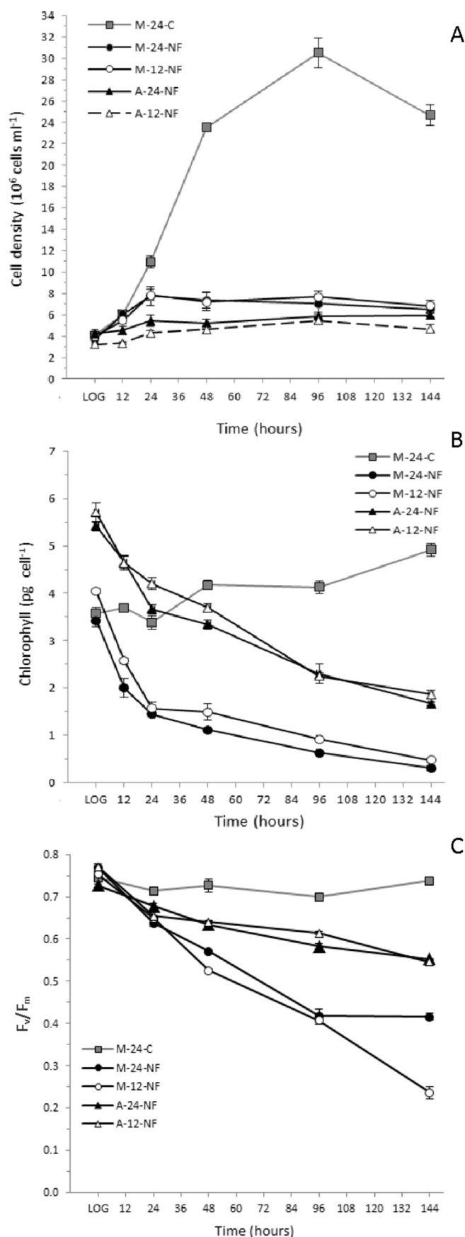
Fig. 3. A). Growth curve of C. reinhardtii after cell resuspension into nitrogen free (NF) or replete (C) medium. B) Chlorophyll concentration ( pg\ cell^{-1} ) before (LOG) and after cell resuspension in nitrogen free (NF) or replete (C). C) Maximum quantum yield of PSII ( F_v/F_m ) before (LOG) and after cell resuspension in nitrogen free (NF) or replete (C) medium. LOG, indicates sampling point at which cells were in the log (exponential) phase of growth, immediately before transfer to N deplete (–N) medium. Treatment conditions are outlined in Table 1, M-24-C, mixotrophic continuous light, C medium; M-24-NF, mixotrophic continuous light NF medium; M-12-NF, mixotrophic diurnal light, NF medium; A-24-NF, autotrophic continuous light, NF medium; A-12-NF, autotrophic diurnal light, NF medium. Error bars represent SE ( n = 3 ).
