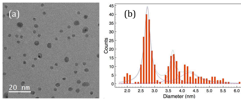
Figure 1 (a) A typical TEM image of the size-selected \text{Au}_{923} clusters deposited onto an amorphous \text{Si}_3\text{N}_4 substrate. (b) Diameter histogram of the Au clusters. The solid line curves are the Gaussian fitting.
