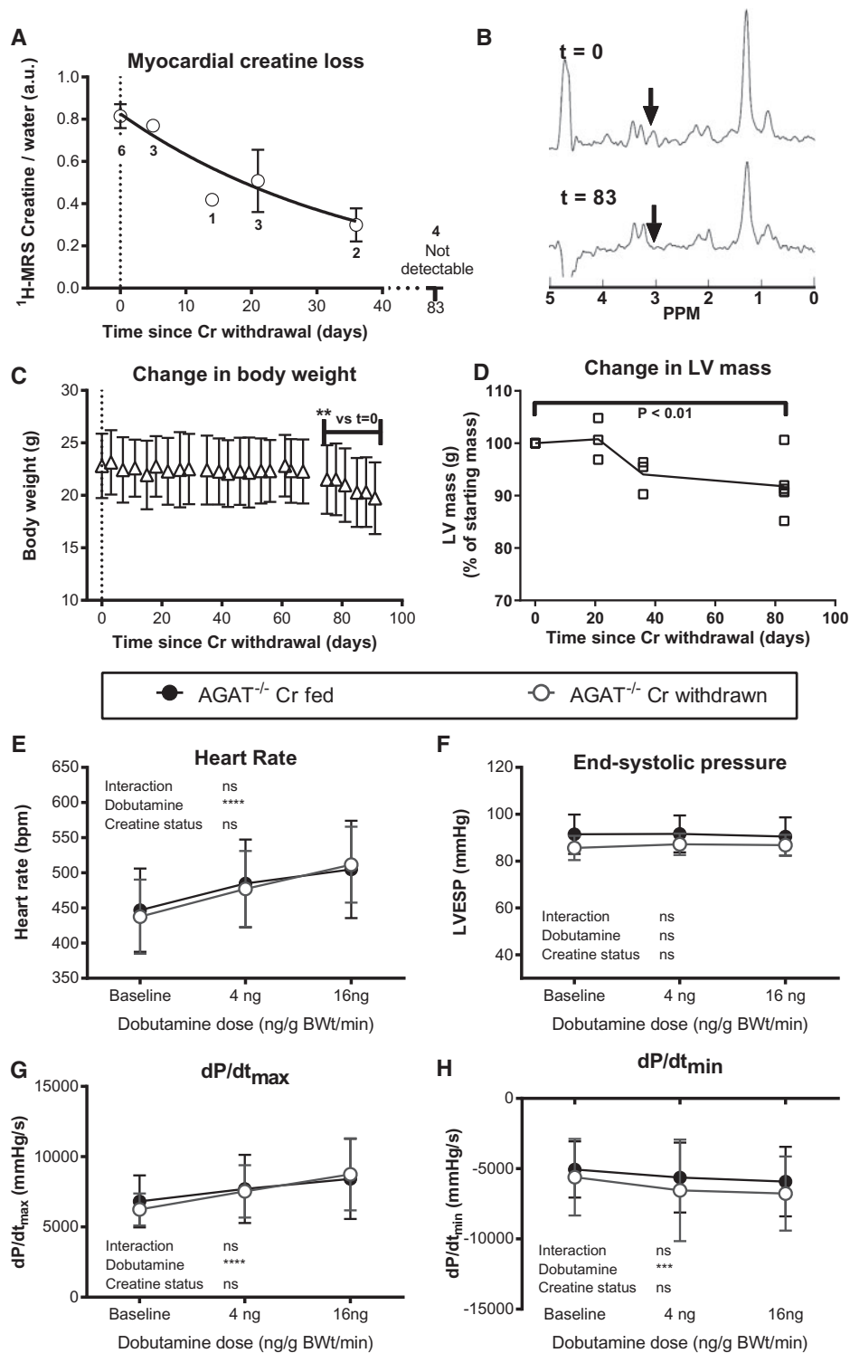
Figure 2 Withdrawal of dietary creatine in AGAT^{-/-} mice reduces body weight and LV mass without affecting haemodynamic function. (A) Myocardial creatine depletion was estimated at 2.7 \pm 0.4\% of the free creatine pool per day using in vivo ^1H -MRS. Data were fitted using a kinetic model of non-enzymatic degradation, according to the following equation: [Cr]_t = [Cr]_{t=0} \cdot e^{-kt} . (B) Representative ^1H -MRS spectra of the same mouse before and after creatine withdrawal. The creatine peak (arrow) seen at day 0 is not visible by day 83. (C) Body weight decreased rapidly after 70 days of creatine-free diet ( n = 6 ). (D) LV mass calculated by in vivo cine-MRI falls during dietary creatine withdrawal. LV haemodynamic parameters were measured at day 90 in AGAT^{-/-} mice with and without dietary creatine withdrawal ( n = 6 /group) under resting baseline conditions and with IV infusion of dobutamine. There were no significant differences between groups for (E) heart rate, (F) LV end-systolic pressure, (G) the rate of pressure rise maximum ( dP/dt_{max} ) as a measure of contractility, or (H) the rate of pressure rise minimum ( dP/dt_{min} ) as a measure of relaxation. Comparison was made by two-way repeated measures ANOVA and data are represented as mean \pm SD.
