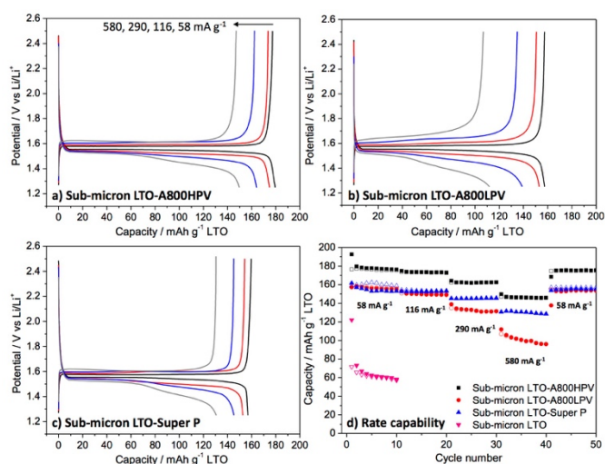
Fig. 9. Galvanostatic charge-discharge voltage profile (1.25 to 2.5 V) of a) Sub-micron LTO-A800HPV, b) Sub-micron LTO-A800LPV and c) Sub-micron LTO-Super P. d) Rate-capability and cycling performances at different current (58, 116, 290 and 580 mA g -1 ). Sub-micron LTO electrodes prepared without any carbon additive tested only until 10 th cycle at 58 mA g -1 . Filled and open symbols refer to reduction (discharge) and oxidation (charge), respectively.
