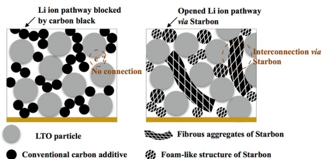
Fig. 7. Schematic representation of LTO electrodes with conventional carbon additive, and with Starbon. (scheme not a scale)
