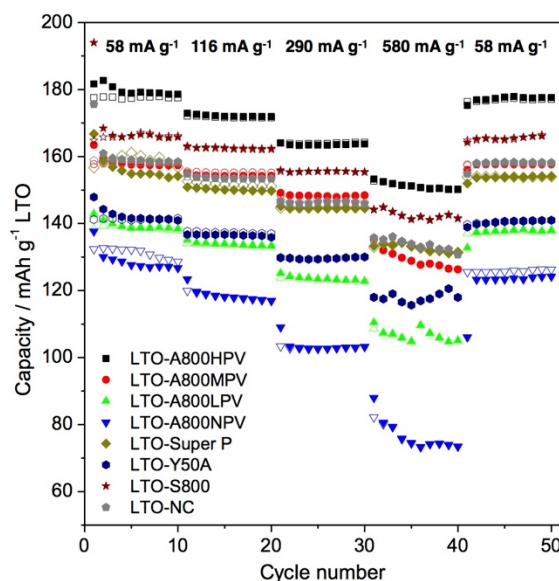
Fig. 3. Rate-capability and cycling performances of LTO electrodes formulated with different carbon additives. Filled and open symbols refer to reduction (discharge) and oxidation (charge), respectively.
