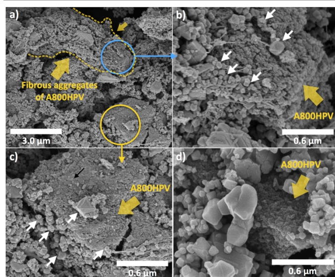
Fig. 6. a), b) and c) Cross-sectional SEM image of LTO-A800HPV electrode, some LTO particles indicated by white arrows. d) Top-view of LTO-A800HPV electrode. More images in Fig. S11 and S12.
