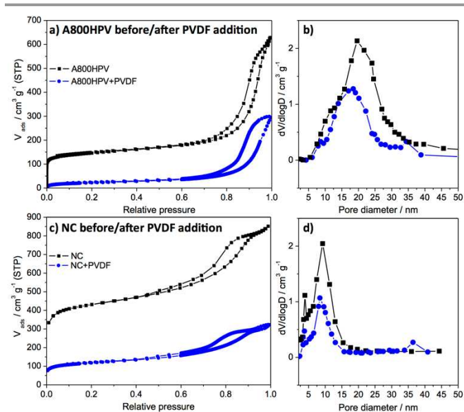
Fig. 5. N_2 adsorption-desorption isotherm for a) A800HPV before/after PVDF addition, b) NC before/after PVDF addition.
