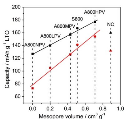
Fig. 4. Specific capacity of LTO electrodes formulated with mesoporous carbons as a function of the mesopore volume of the carbon additive. Black and red symbols refer to capacity measured at current densities of 58 and 580 mA g -1 , respectively.
