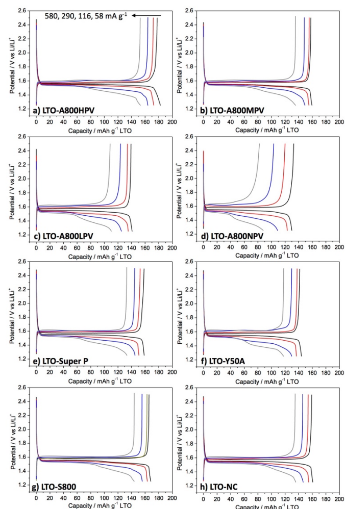
Fig. 2. Galvanostatic charge-discharge voltage profiles (1.25 to 2.5 V) of LTO electrodes formulated with different carbon additives: a) LTO-A800HPV, b) LTO-A800MPV, c) LTO-A800LPV, d) LTO-A800NPV, e) LTO-Super P, f) LTO-Y50A, g) LTO-S800, and h) LTO-NC.
