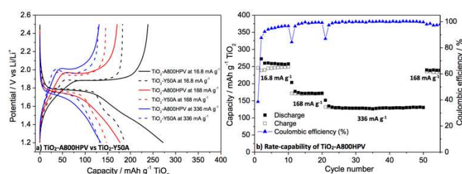
Fig. 10. a) Galvanostatic charge-discharge voltage profiles (1.2 to 2.5 V) of TiO 2 -A800HPV and TiO 2 -Y50A; b) Rate-capability and cycling performances of TiO 2 -A800HPV. Filled and open symbols refer to reduction (discharge) and oxidation (charge), respectively.
