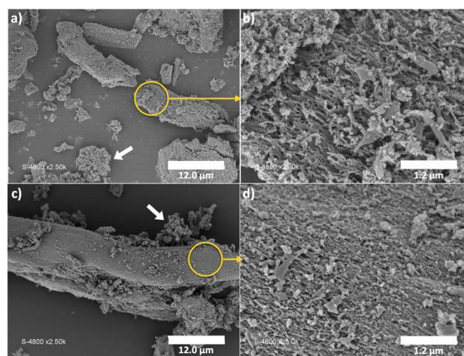
Fig. 1 SEM image of a) A800HPV, b) zoomed image of selected zone of A800HPV (fibre-like aggregates), c) A800LPV and d) zoomed image of selected zone of A800LPV (fibre-like aggregates); foam-like aggregates indicated by white arrow. For other carbon additives, such as A800MPV or Super P, see Fig. S6.
