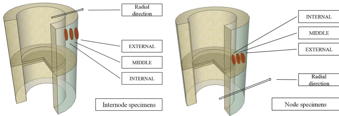
Fig 2. The cutting position of bamboo specimens in the radial direction
