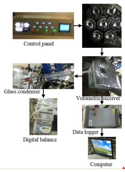
Fig. 33 Schematic of the experimental setup highlighting the major components.
