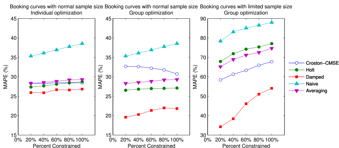
Figure 4: Accuracy for best performing methods (optimized on groups) for different restriction scenarios.
