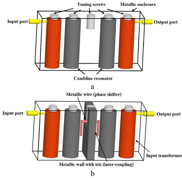
Fig. 6. Geometrical structure of combline filters (a) Positive coupling introduced via an iris/window, (b) Negative coupling (phase shifter) achieved by an opening in the upper part of the wall and a metallic wire suspended in the iris between the resonators
