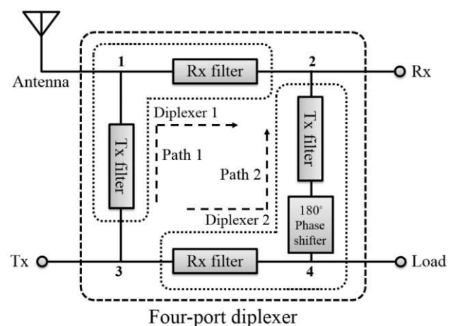
Fig. 1. Schematic diagram of four-port diplexer using two back-to-back three-port diplexers with amplitude and 180° phase cancellation technique between Rx and Tx channel
