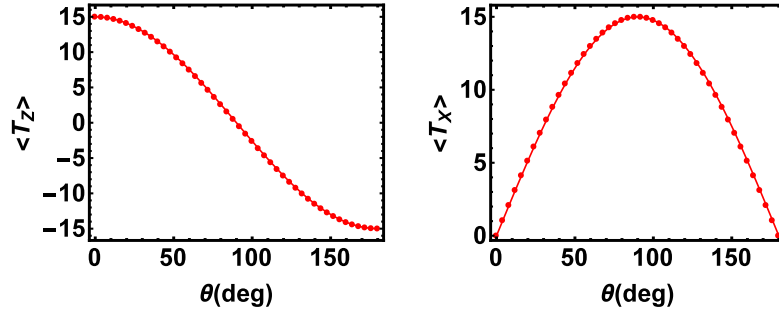
Fig. 2. First and third components of the isospin as functions of \theta , obtained for l = 10 , A = 36 , and x = 0 , for an isoaligned state with \langle \hat{T}_z \rangle \Big|_{\theta=0} = 15
