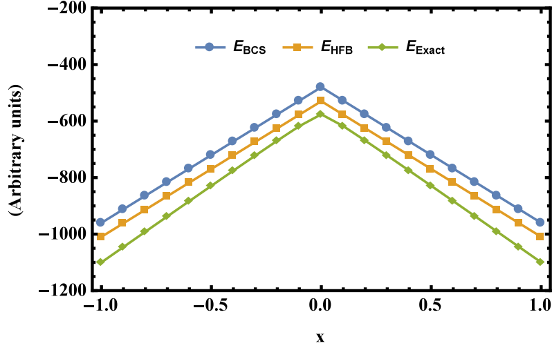
Fig. 1. Total energies (in arbitrary units) as functions of the mixing parameter x , obtained from the HFB (squares), generalized BCS (circles), and exact solutions (diamonds) with l = 15 , A = 64 , and \langle \hat{T}_z \rangle = \langle \hat{T}_x \rangle = 0 .
