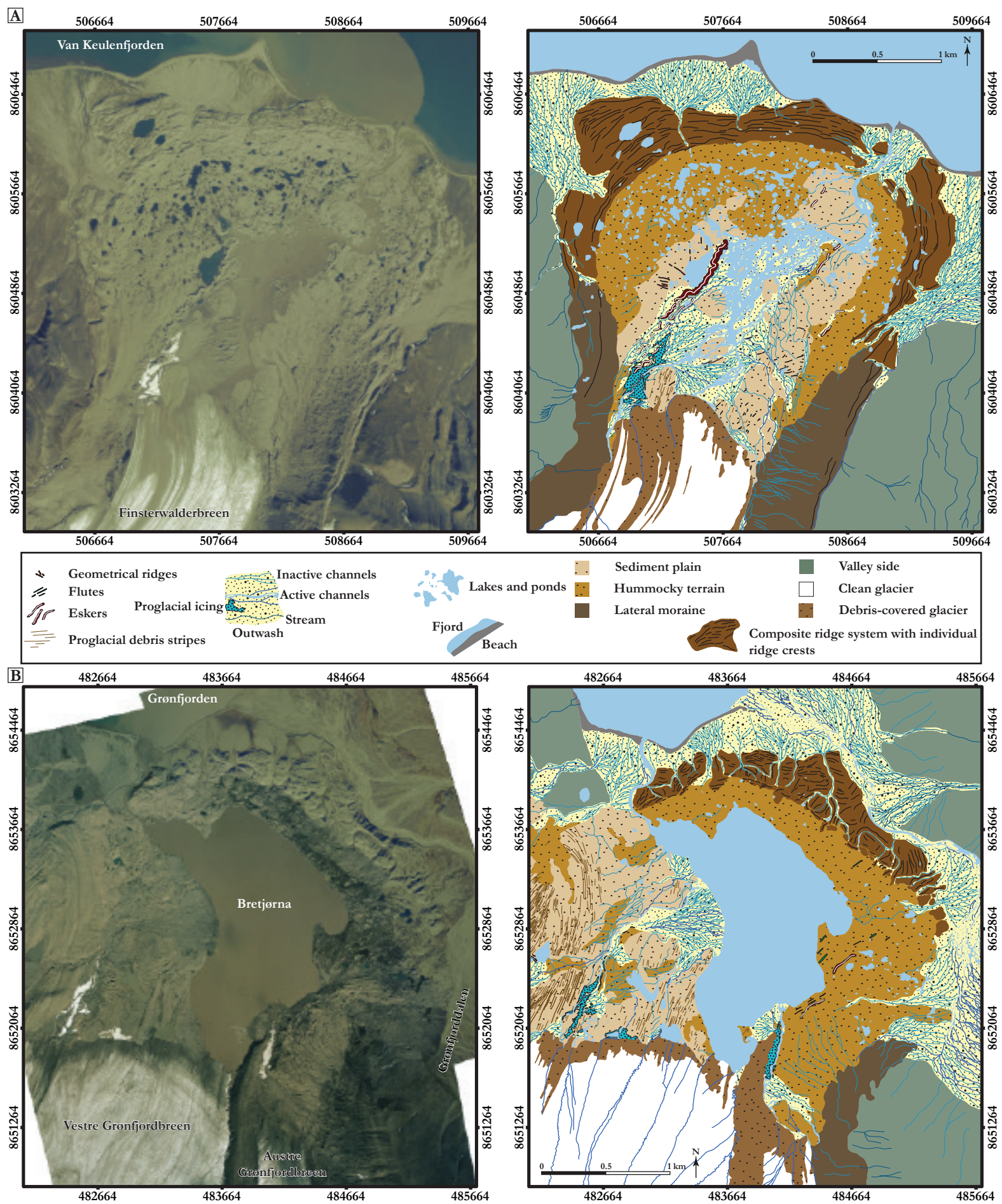
Fig. 4. Aerial photographs and geomorphological maps of (A) Finstervalderbreen and (B) Grønfjordbreen.
