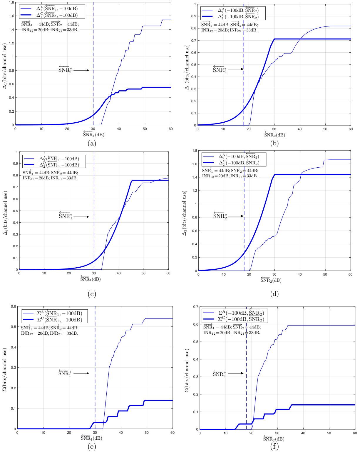
Fig. 6. Improvement metrics \Delta_i^A , \Delta_i^C , \Sigma^A , and \Sigma^C as functions of \overline{\text{SNR}}_1 and \overline{\text{SNR}}_2 , with i \in \{1, 2\} , for Example 4.
