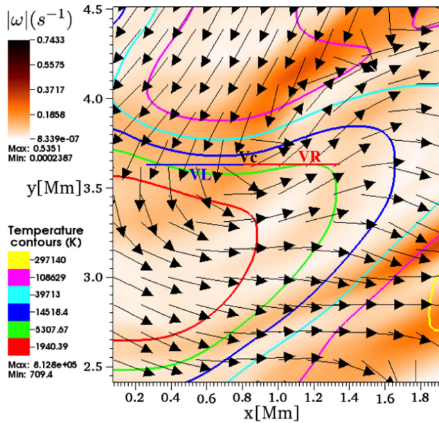
Figure 12. (Left) Region where the Doppler shift \Delta v_D is estimated. This is a zoomed-in view of a vortex region of Figure 11 at time t = 60 s. (Right) Value of \Delta v_D of the y component of velocity v_y , or equivalently the tangent velocity, as a function of distance from the center.
