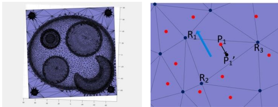
(a) CAD model of NPL artefact (b) Normal-vector-based method
