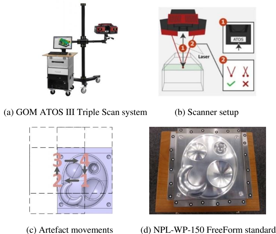
Fig. 2. Measuring equipment & setup
