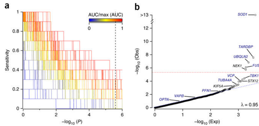
Figure 1. RVB analysis of FALS exomes. (a) RVB analyses of 1,022 index FALS cases and 7,315 controls for 10 known ALS genes, to assess 308 different combinations of MAF and functional prediction filters (Supplementary Table 1). The set of analysis parameters achieving the highest sensitivity for known ALS genes was identified as that achieving the highest area under the curve (AUC) in a plot of sensitivity (proportion of training genes achieving significance) across an increasing minimum P -value threshold. Dotted vertical line denotes Bonferroni-corrected P value for exome-wide significance. (b) Extension of the highest performing known gene-trained analysis to the entire exome. Threshold for exome-wide significance is denoted by the dotted red line. \lambda , observed genomic inflation factor. ‘Obs’ describes the P -value distribution for the observed data. ‘Exp’ describes the P -value distribution under null expectation.
