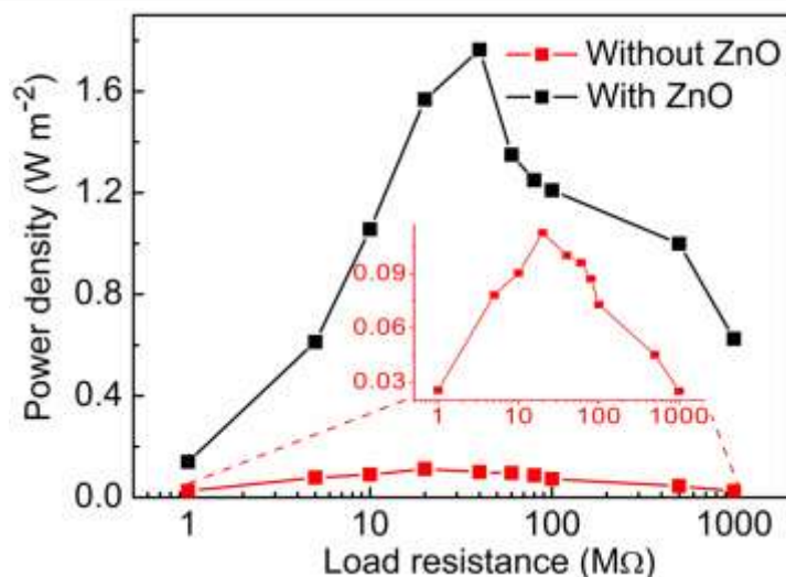
Fig. 5. Comparison of output power density vs. load, showing the maximum power outputs for samples S3 and S4 at \sim 20 M \Omega and \sim 40 M \Omega , respectively. The inset shows the blow-up of the power vs. load curve for sample S3.
