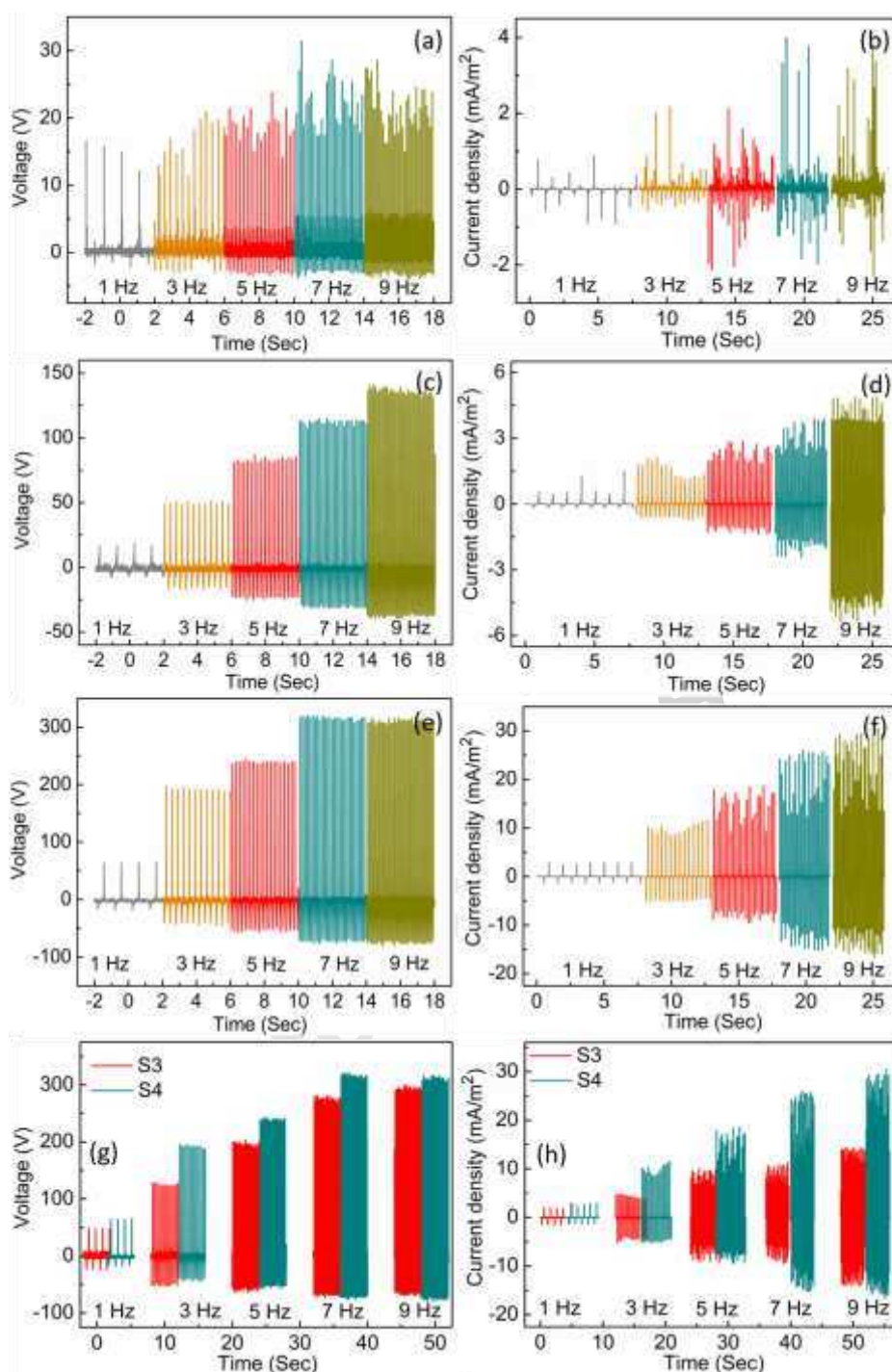
Fig. 4. (a) Open circuit voltage ( V_{oc} ) and (b) short circuit current densities ( J_{sc} ) of sample S1, corresponding V_{oc} and J_{sc} values (c) and (d) for sample S2, while (e) and (f) show the V_{oc} and J_{sc} values for sample S4. The effect of an interfacial ZnO nanosheet layer is best illustrated in the variation of (g) V_{oc} and (h) J_{sc} values for samples S3 and S4. All measurements were carried out at a constant force of 50 N and spacer distance of 8 mm.
