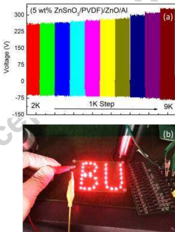
Fig. 6. (a) The stability test of TENG sample S4 carried out for 9000 cycles at a force of 30 N at a driving frequency of 5 Hz, (b) lighting a group of 35 red LED's with as fabricated TENG device by charging a 1 \mu F capacitor.
