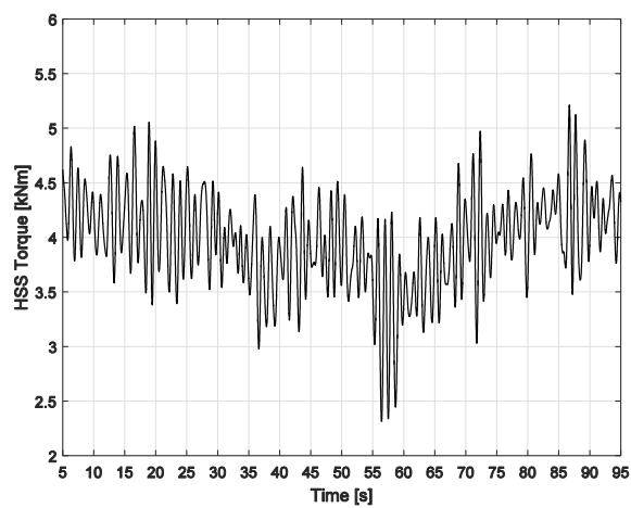
Figure 8. HSS torque - normal operation
