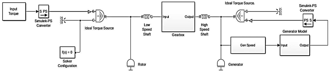
Figure 5. Configuration of MATLAB/Simulink of eleven mass model of the drivetrain
