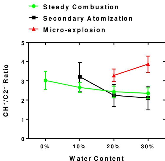
Figure 2 The CH^*/C_2^* ratio for the cases shown in Fig. 5.
