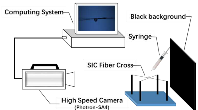
Figure 2 Experimental Setup.
