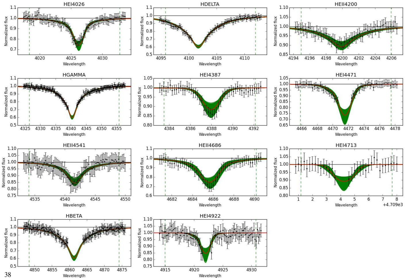
Fig. E.9. Observed spectra, the 95% probability models (green) and the best fit model (red) for VFTS 131 and 142. The vertical dashed lines indicate the wavelength range used to fit the corresponding diagnostic line. [Color version available online.]
