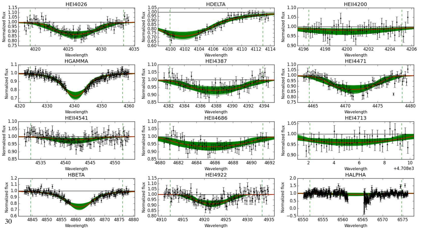
Fig. E.1. Observed spectra, the 95% probability models (green) and the best fit model (red) for VFTS 016 and 035. The vertical dashed lines indicate the wavelength range used to fit the corresponding diagnostic line. [Color version available online.]
