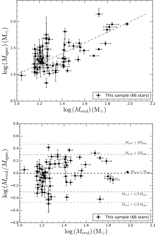
Fig. 11. Comparison of spectroscopic masses and evolutionary masses for the 66 sources that have M_{\text{evol}} constrained by BONNSAI. The upper panel shows a one-to-one comparison; the lower panel shows the ratio of the masses.
