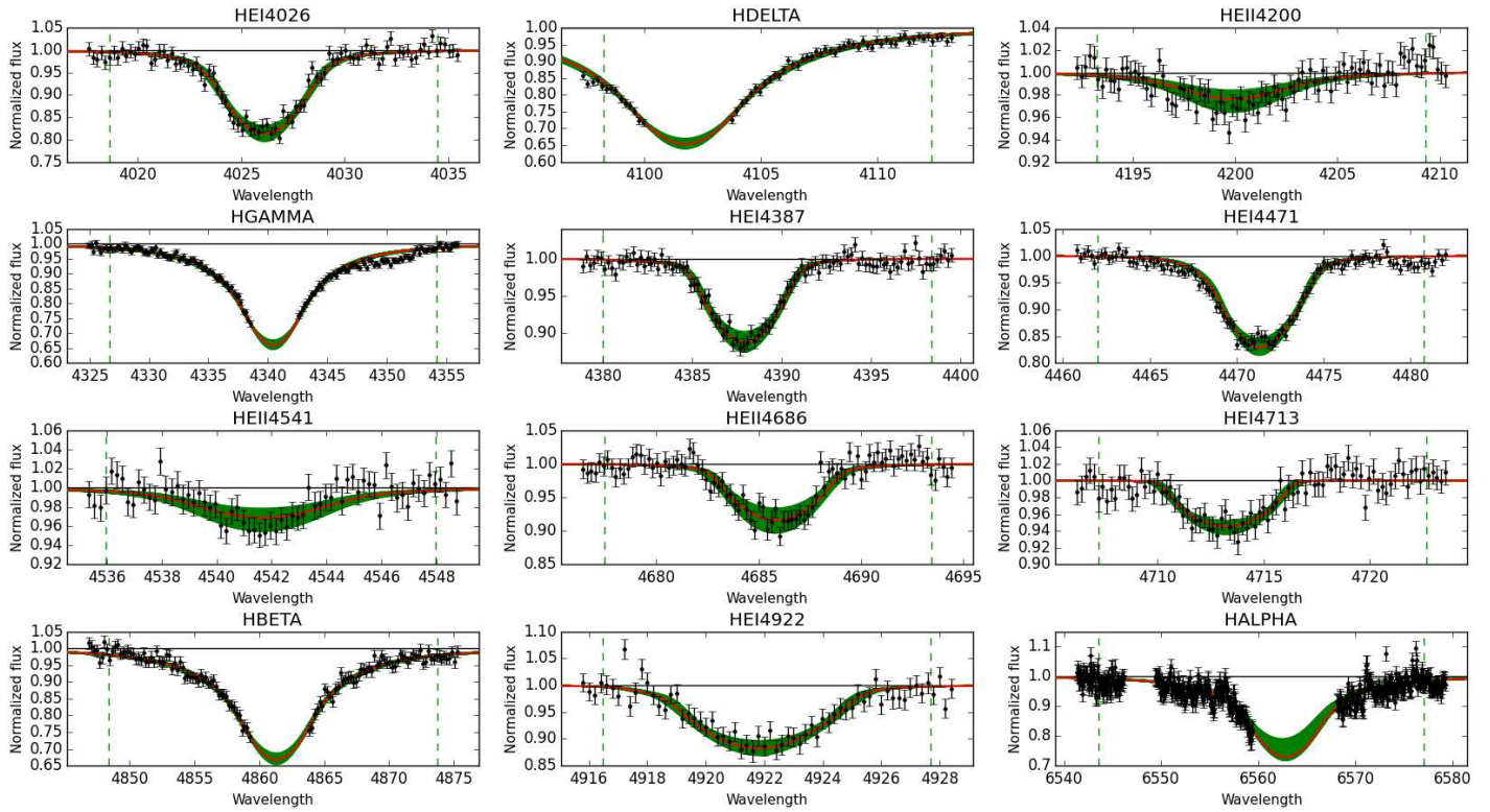
Fig. E.4. Observed spectra, the 95% probability models (green) and the best fit model (red) for VFTS077 and 080. The vertical dashed lines indicate the wavelength range used to fit the corresponding diagnostic line. [Color version available online.]
