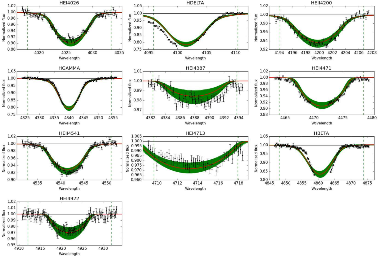
Fig. E.10. Observed spectra, the 95% probability models (green) and the best fit model (red) for VFTS 145 and 177. The vertical dashed lines indicate the wavelength range used to fit the corresponding diagnostic line. [Color version available online.]
