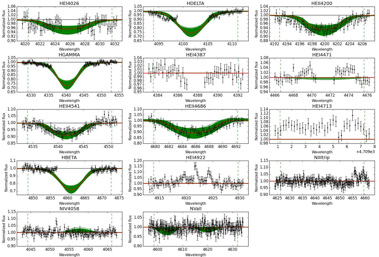
Fig. E.8. Observed spectra, the 95% probability models (green) and the best fit model (red) for VFTS 051 and 125. [Color version available online.]
