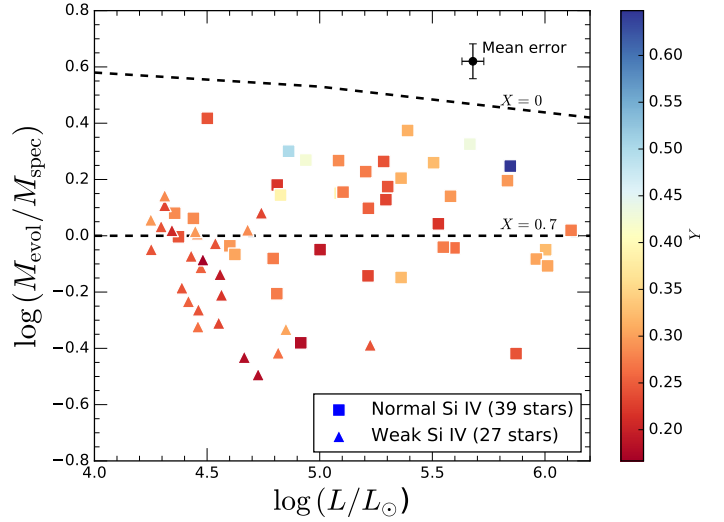
Fig. 12. Mass discrepancy plotted against luminosity for the 66 sources that have M_{\text{evol}} constrained by BONNSAI. The upper dashed line is from the L(M) relation of helium stars; see main text for discussion. The lower line is M_{\text{spec}} = M_{\text{evol}} , and is a lower limit as stars cannot be under-luminous. The color denotes the surface helium abundance. Squares denote stars for which the LC is certain and triangles refer to the sources with weak Si IV relative to He I and for which the luminosity class may be debated (they may be dwarf stars). Helium enriched sources are all positioned above the one-to-one relation.
