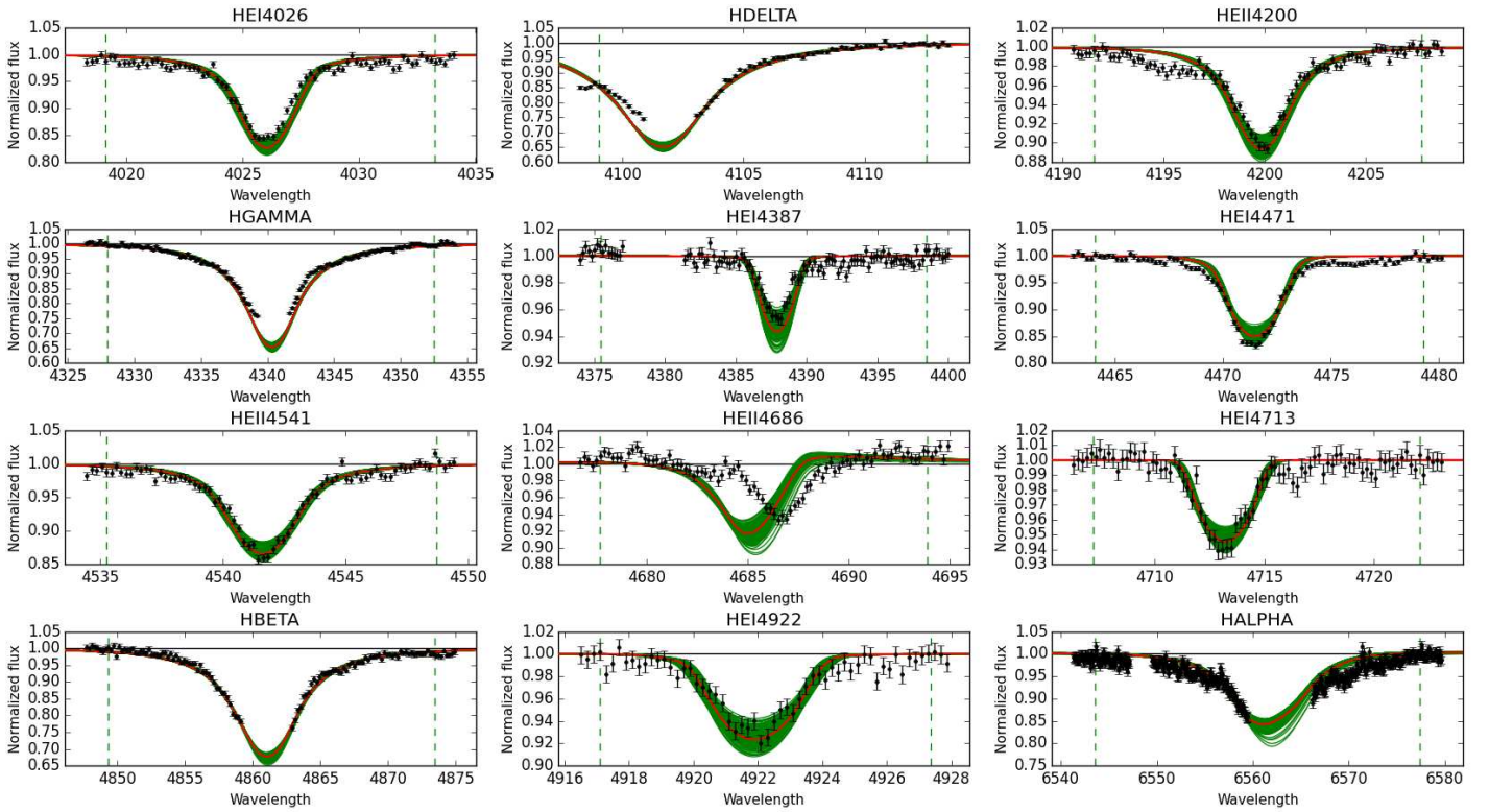
Fig. E.2. Observed spectra, the 95% probability models (green) and the best fit model (red) for VFTS046 and 064. The vertical dashed lines indicate the wavelength range used to fit the corresponding diagnostic line. [Color version available online.]
