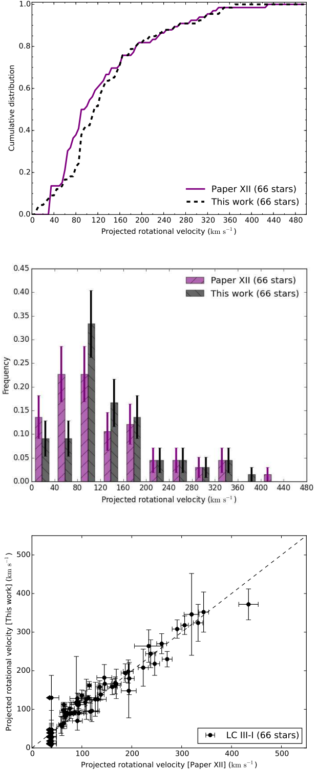
Fig. A.1. Cumulative (upper panel) and frequency (middle panel) distributions of the projected rotational velocities of the O-type LC III to I as derived here from the automated FASTWIND analysis and Paper XII. The middle panel shows Poissonian error bars. The lower panel compares the actual v_e \sin i of these two samples.
