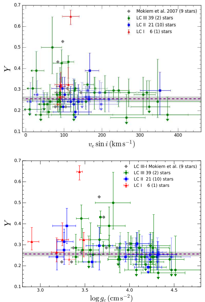
Fig. 7. Helium mass fraction Y versus v_e \sin i (upper panel) and \log g_c (lower panel). Symbols and colors have the same meaning as in Fig. 5. Gray diamonds denote stars with LC III to I from Mokiem et al. (2007a). The purple dashed line at Y = 0.255 defines the initial composition for LMC stars; the gray bar is the 3\sigma uncertainty in this number.
