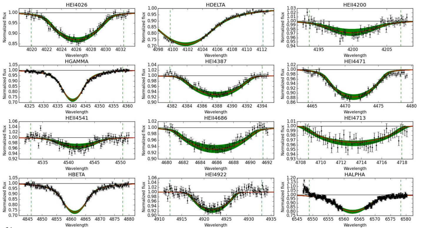
Fig. E.5. Observed spectra, the 95% probability models (green) and the best fit model (red) for VFTS087 and 091. The vertical dashed lines indicate the wavelength range used to fit the corresponding diagnostic line. [Color version available online.]
