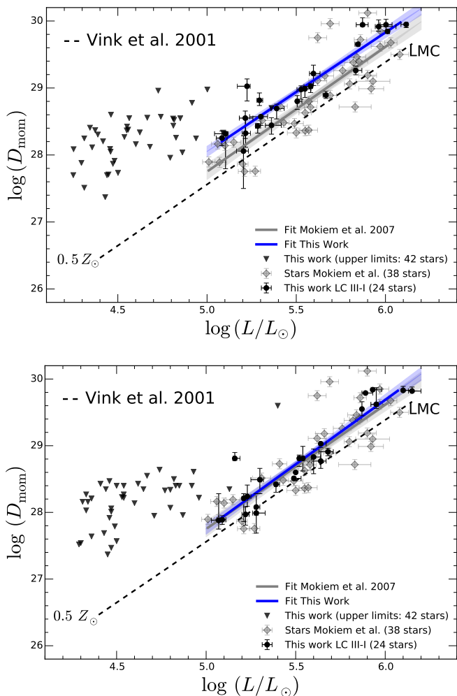
Fig. 10. Modified wind momentum ( D_{\text{mom}} ) vs. luminosity diagram. The dashed lines indicate the theoretical predictions of Vink et al. (2001) for homogeneous winds. Top panel: the empirical fit for this work and Mokiem et al. (2007a) (both for L/L_{\odot} > 5.0 ) in shaded blue and gray bars, respectively. For stars with L/L_{\odot} \leq 5.0 , only upper limits could be constrained. These stars are not considered in the analysis. Bottom panel: same as top panel but now for an analysis in which the acceleration of the wind flow, \beta , is a free parameter and in which the analysis does not include nitrogen lines, but relies on hydrogen and helium lines only. [Color version available online].
