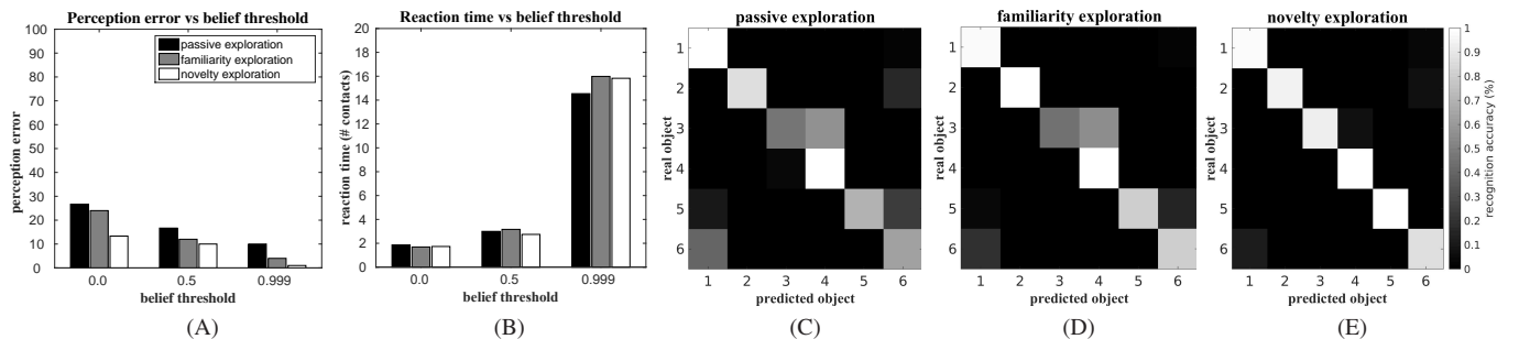
Fig. 6. Perception error and reaction time results, averaged over all test objects from real world experiments for passive and active exploration behaviours. (A) Perception error decreased, achieving small values, for active exploration behaviour. Exploration of locations with high (novelty) levels of interestingness achieved the best perception. (B) Reaction time increased for larger values of belief threshold. Similar reaction times were observed for both passive and active exploration. Confusion matrices from object recognition results with passive (C) and active (D, E) exploration. The test objects used for the experiments are: 1) triangle, 2) cylinder, 3) blue 1, 4) ball 2, 5) box 1 and 6) box 2. Even though improvements were achieved by all the exploration behaviours, the best performance was obtained with the novelty approach, which explored the locations with high levels of interestingness.
